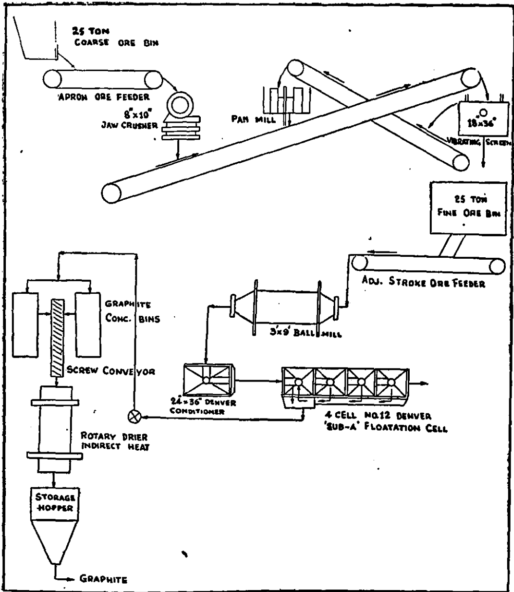
FLWSHEET FOR CONCENTRATION OF GRAPHITE.
