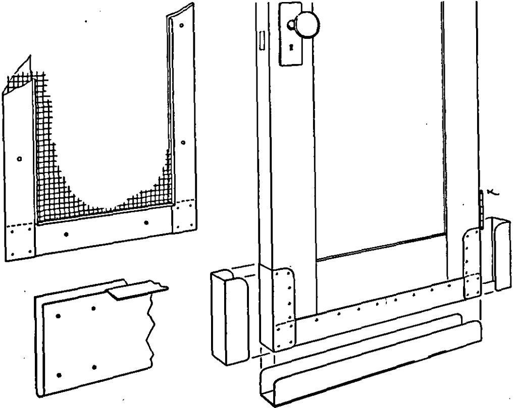
Fig. 8.—Permanent rat-proofing for windows and doors. Left , four folded channels of galvanized sheet iron are bent to cover edges of hardware cloth (3 meshes per inch); a narrow lip ( \frac{3}{16} to \frac{1}{4} inch) is bent out along one margin of each channel to stiffen the frame; the 4 channels are riveted together at the corners and the framed screen is fastened to the window casing with screws. An enlarged detail of the channel is shown below. Right , three rectangular channels are bent from galvanized sheet iron to fit closely around the bottom and lower edges of a door and nailed or screwed into place. These channels add strength to the door, they prevent damage to the lower edge, and they will stay in position much better than flat strips of sheet metal tacked to one side of the door.
