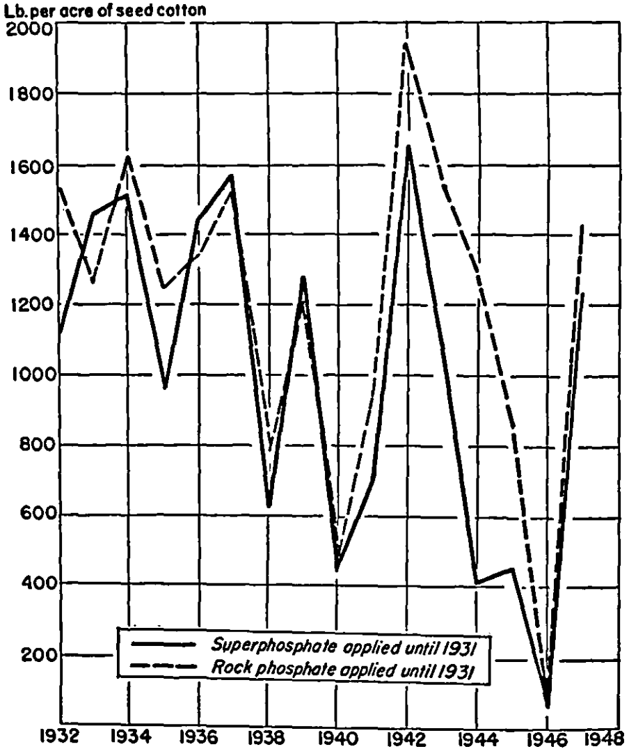
FIGURE 1. The effect of residual phosphate on the yield of cotton grown in Collars rotation at Auburn. The superphosphate plots received a total of 914 pounds per acre of P_2O_5 from 1911 to 1931. The rock phosphate plots received a total of 3,656 pounds per acre of P_2O_5 during the same period.
