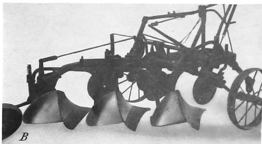
FIGURE 23.—Three-bottom, 18-inch plow equipped with adjustable hinged-type moldboards. A , Moldboards in the forward position; B , in the rear position.
