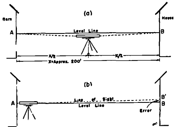
Figure 8. Level line method (a) First step. (b) Second step.
