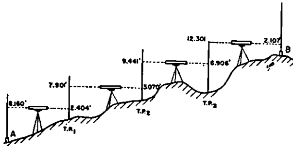
Figure 10. Diagram illustrating differential leveling.
