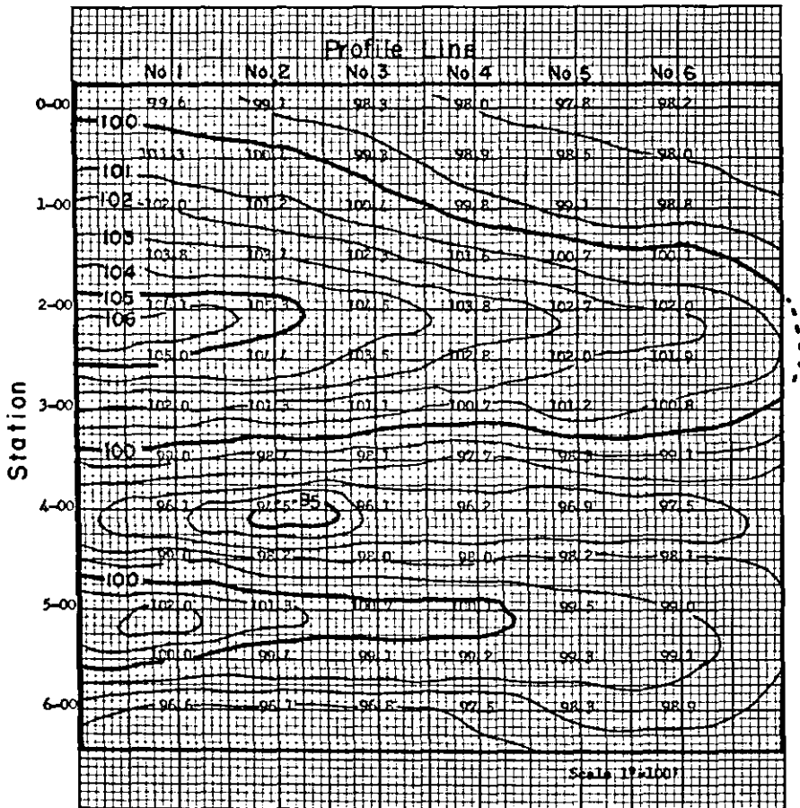
Figure 13. Contour map using notes in Table III.
