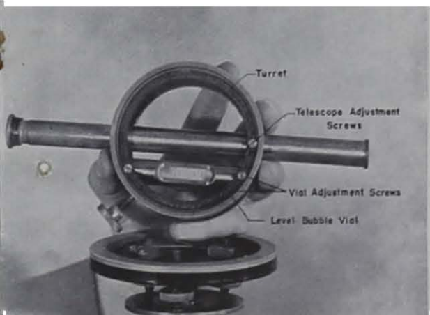
Figure 6. Turret removed showing the bubble vial adjustment screws.
