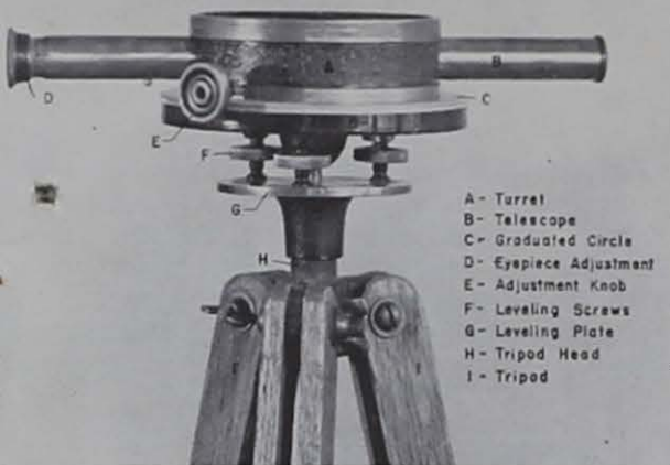
Figure 3. Turret type level showing parts.
