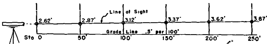
Figure 11. Running a grade line.
