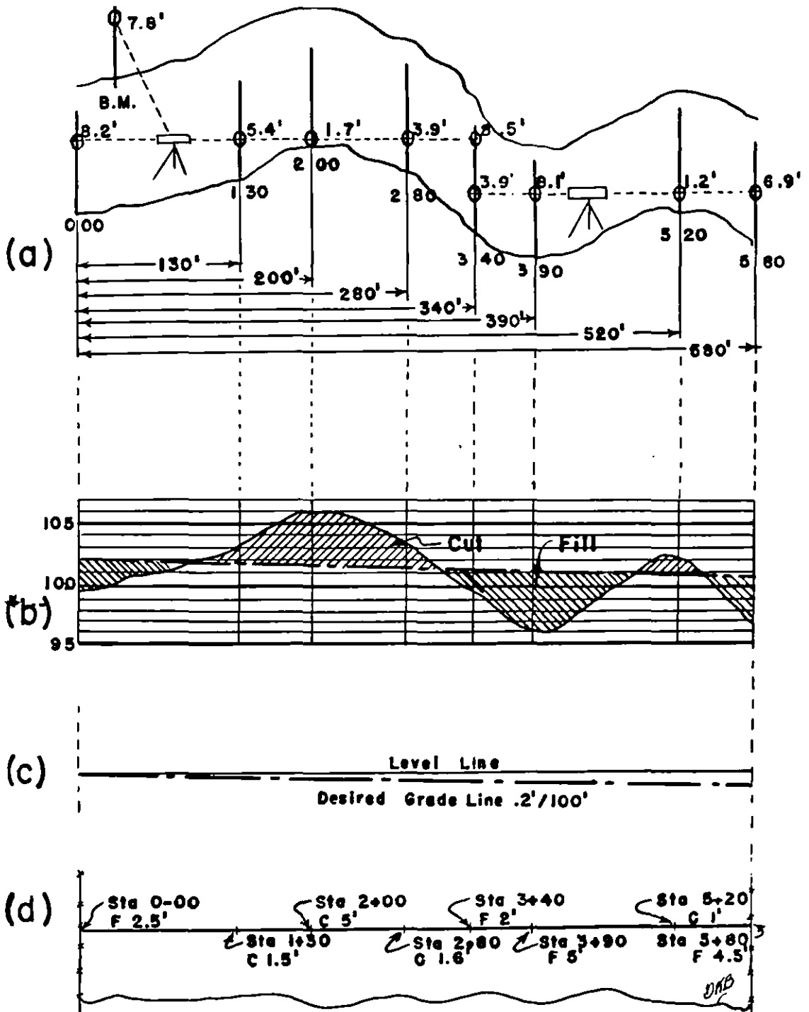
Figure 12. Plotting the notes from Table II.
