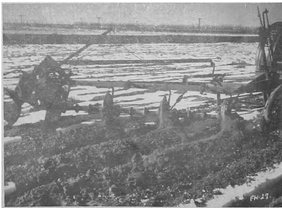
Figure 8.—A "frozen soil" lister can be readily fashioned from a one-way disk. This implement is very effective in stopping winter drifting.
