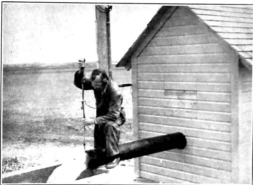
Figure 6.—Making discharge measurement with Hoff current meter. Pump is the turbine type in a shelter typical of the region.
