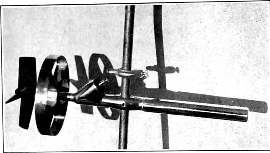
Figure 5.—Hoff current meter with guard for measuring flow in pipes.
