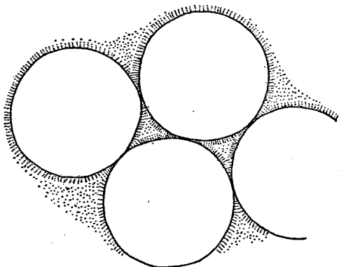
FIG. 3. Structure of a colloidal gel, diagrammatic and magnified about 200,000 times.
