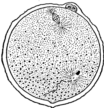
FIG. 5. Fertilization of an animal ovum, magnified 250 times.
