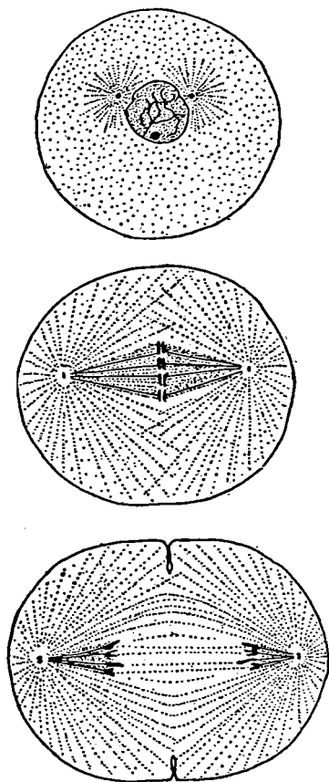
FIG. 2. Cell division : prophase, metaphase, and anaphase.
