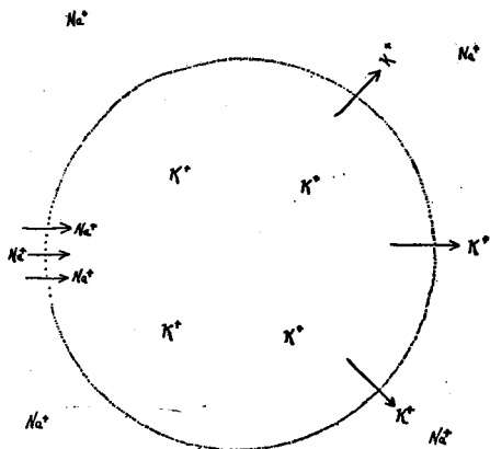
FIG. 4. Diagram illustrating electric currents in living cells.
