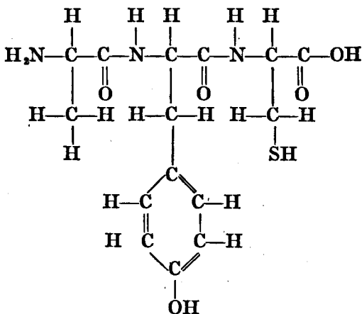
alanyl-tyrosinyl-cysteine, \text{C}_{16}\text{H}_{25}\text{N}_3\text{SO}_8 .
