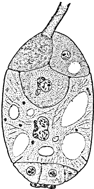
FIG. 7. Fertilization in a flowering plant, 300 times magnified.
