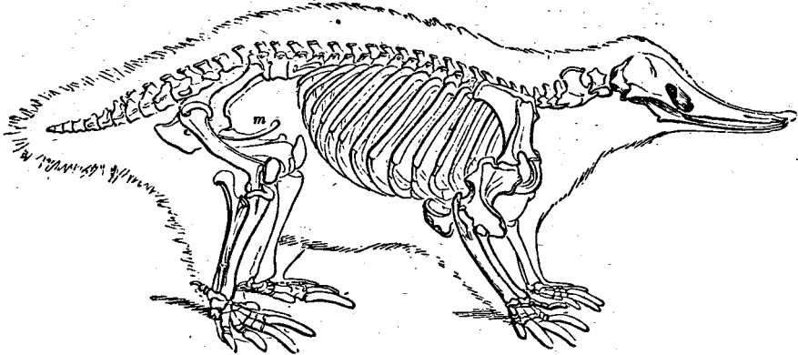
FIG. 60.—Spiny Ant-eater.
