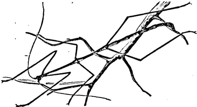
FIG. 72.—Walking-stick Insect.
