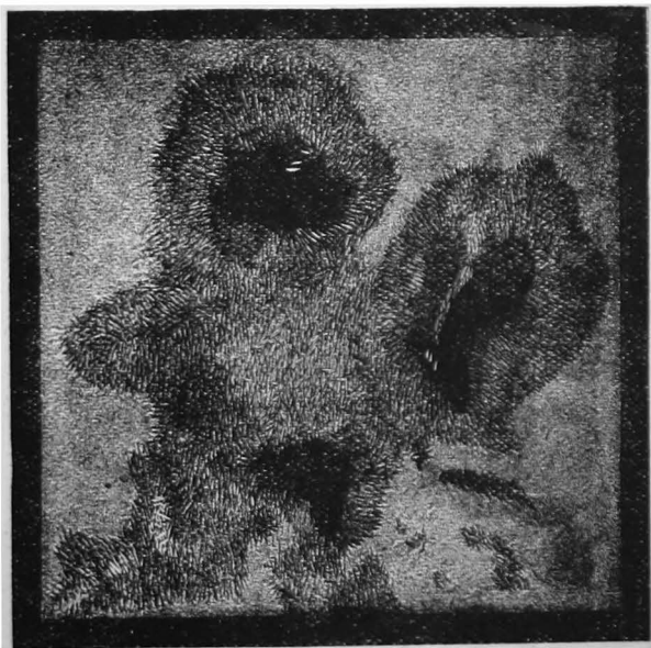
FIG. 1.—Sun-spots.
