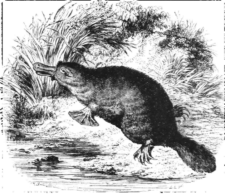
FIG. 59.—Duckbill.
