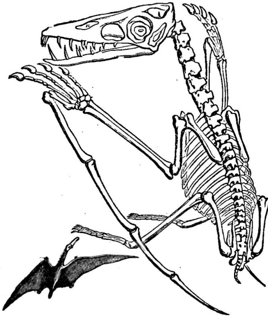
FIG. 16.—Pterodactyl (Wing-finger).
