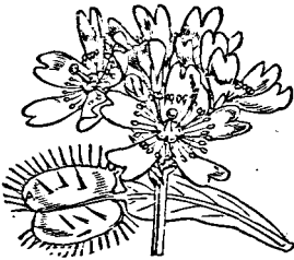
FIG. 26.—Venus's Fly-trap.
