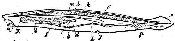
FIG. 56.—Lancelet.
