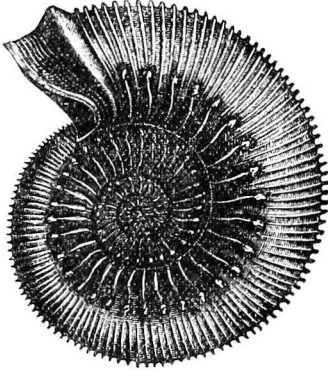
FIG. 18.—Ammonite.
