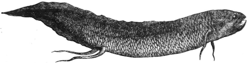
FIG. 57.—Mud-fish.
