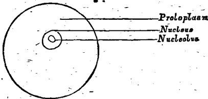
FIG. 65.—Cell.
