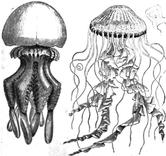
FIG. 40—Jelly-fish.
