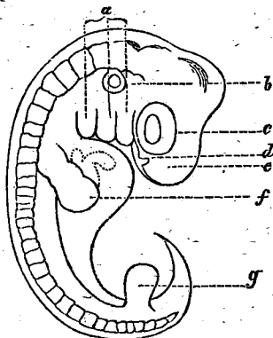
FIG. 76.—Tortoise (4 weeks).
