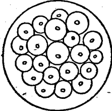
FIG. 67.—Morula Stage.
