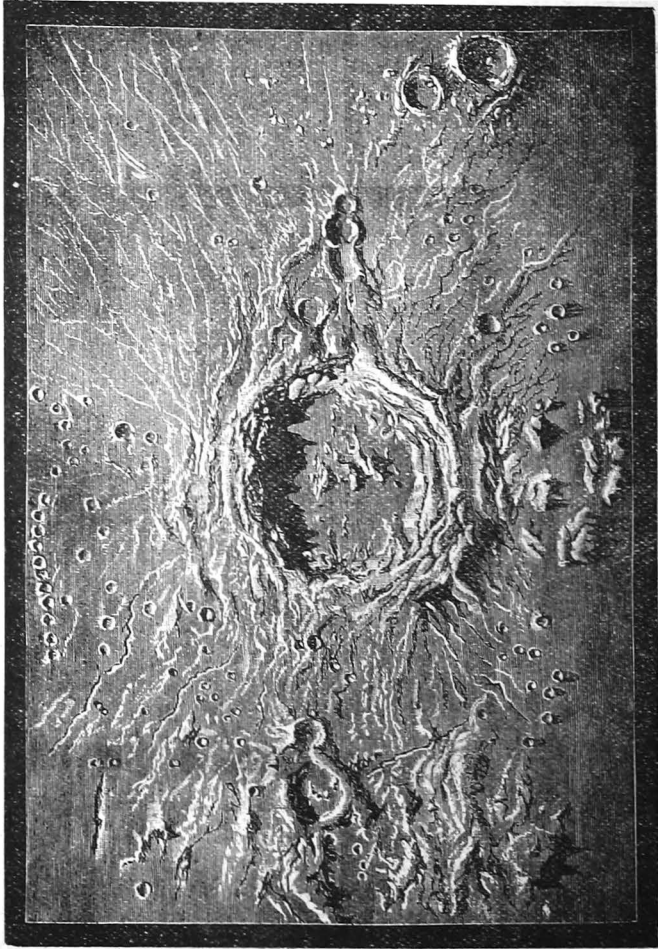
FIG. 2.—Lunar Crater : Copernicus.
