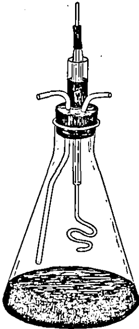
Fig. 2. Flask fitted with mercury seal stirrer.
