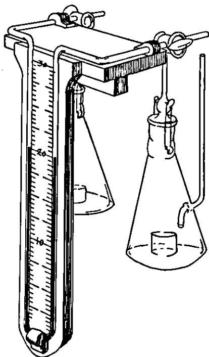
Fig. 3. Modified Barcroft differential manometer.
