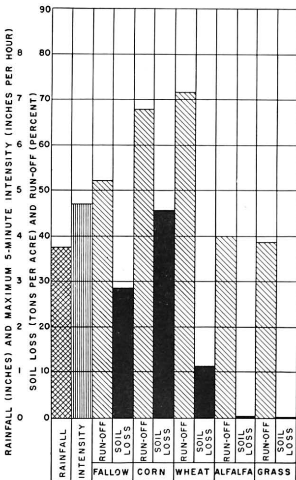
FIGURE 9.—Effect of plant cover on run-off and soil loss on an 8-percent slope during rain of high intensity, April 3, 1934, at Bethany, Mo.
