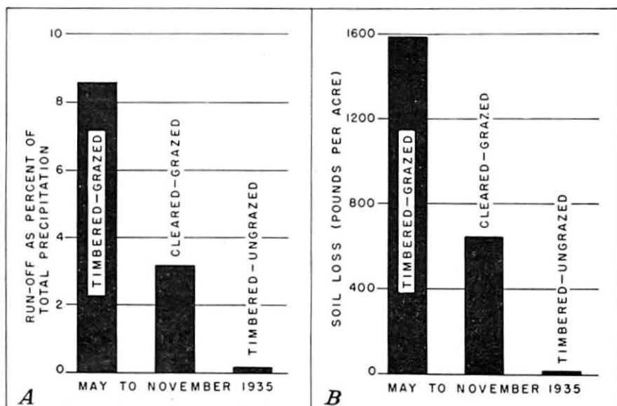
FIGURE 16.—During the eight most intense rains at La Crosse, Wis., run-off (A) and soil loss (B) occurred only twice from an ungrazed wooded watershed, and then in quantities so small as to be insignificant.
