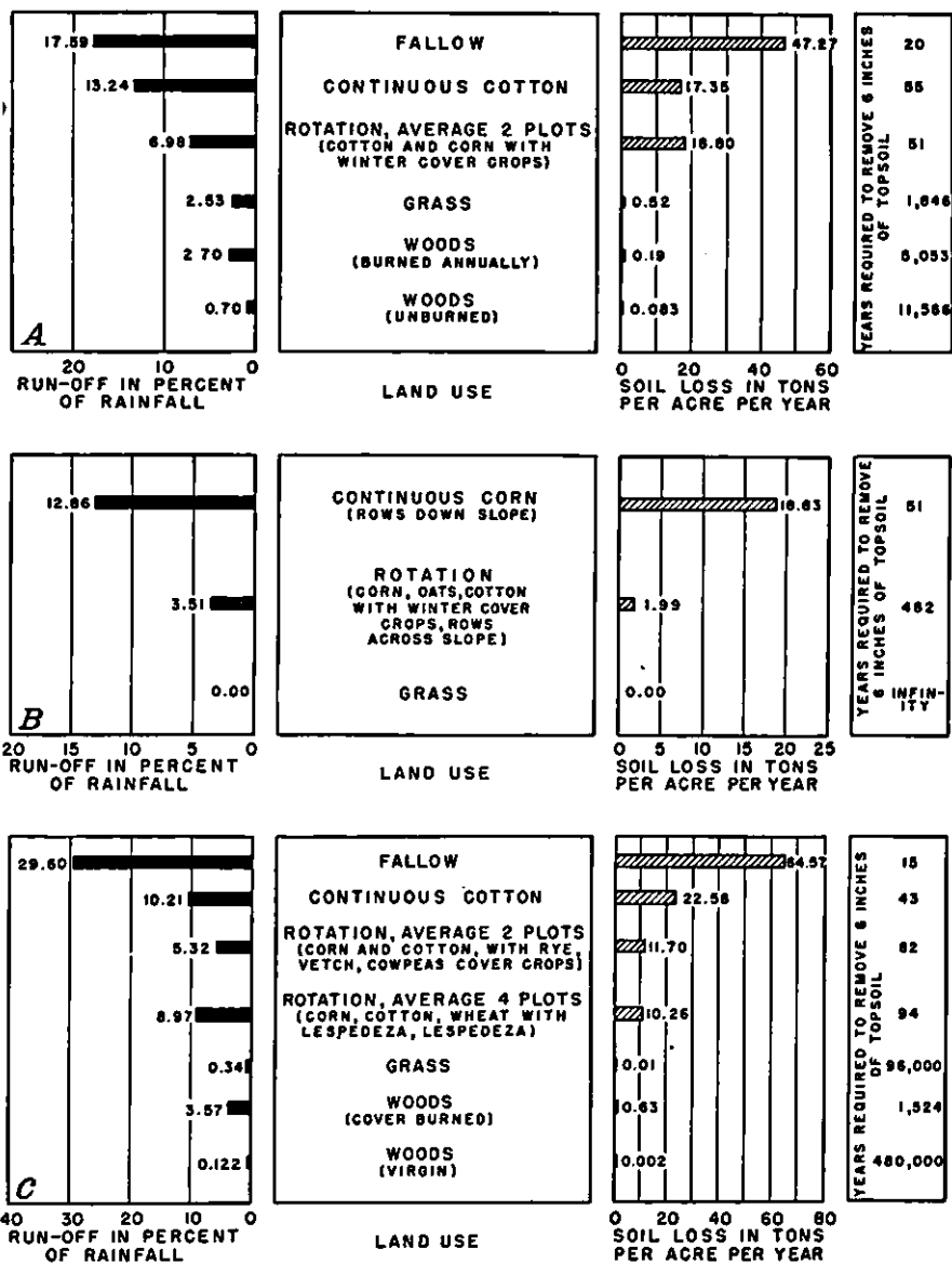
FIGURE 20.—Effect of crop rotation in retarding run-off and soil erosion under various conditions: A , Statesville, N. C., Cecil sandy clay loam, 10-percent slope, average annual rainfall of 45.22 inches, 5-year period 1931-35; B , Temple, Tex., Houston black clay, 4-percent slope, average annual rainfall of 27.51 inches, 4-year period 1931-34; C , Tyler, Tex., Kirvin fine sandy loam, 8½-percent slope, average annual rainfall of 40.52 inches, 4-year period 1931-34.
