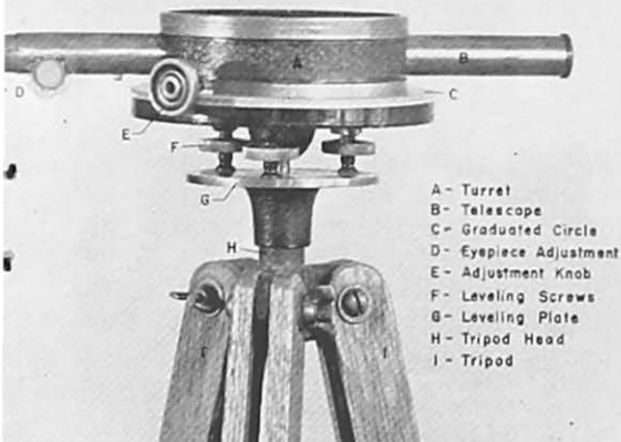
Figure 3. Turret type level showing parts.
