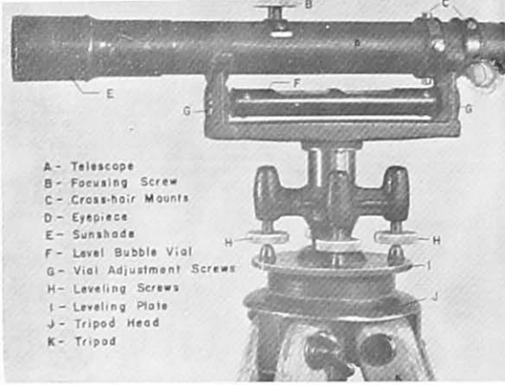
Figure 2. Utility type level showing parts.
