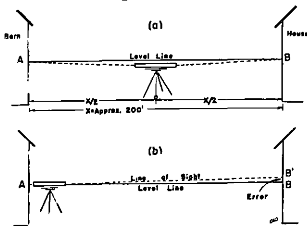
Figure 8. Level line method (a) First step. (b) Second step.
