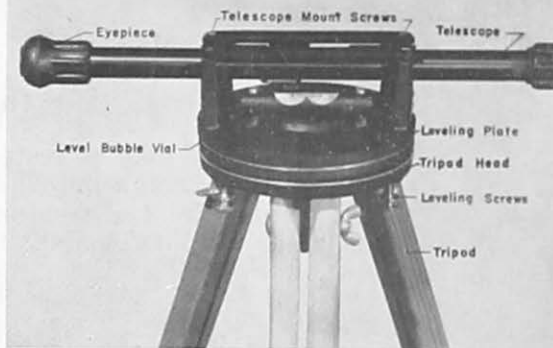
Figure 4. Gunscope type level showing parts.
