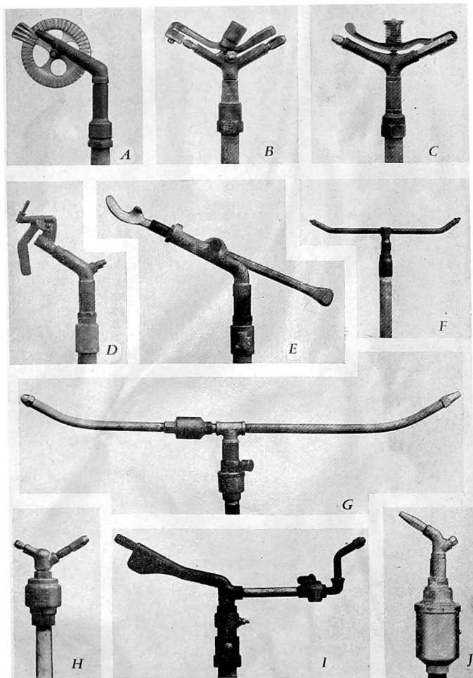
Fig. 1. Some types of rotating sprinklers. A, B, C, D, and E , sprinklers with external driving mechanisms: A , spinning-wheel type; B and C , oscillating spring type; D and E , pendulum type. F , reaction-drive whirling sprinkler. G and I , reaction drive with vibrator for slow rotation. H and J , internal-drive sprinklers: H , friction type; and J , gear type.
