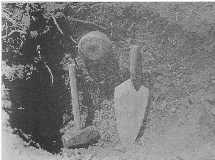
FIGURE 12.—Each volume-weight soil sample was obtained by driving a 4-inch cylinder into a vertical face of undisturbed soil.
