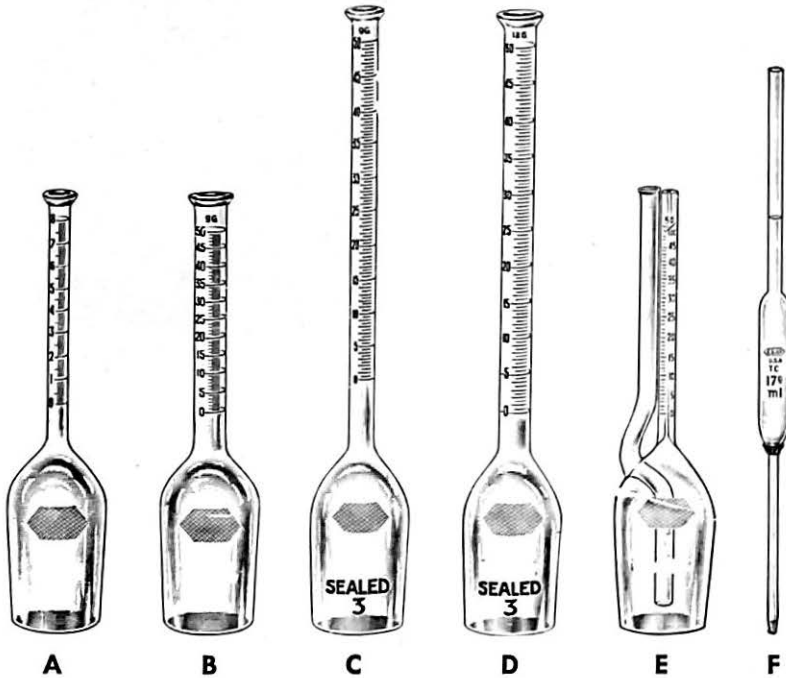
Test bottles for milk and cream and a milk pipet. (A) Milk test bottle, 18-gram, 6-inch, graduated in .1% from 0 to 8%. (B, C, D) Cream test bottles graduated in .5% from 0 to 50%. B is a 9-gram, 6-inch bottle; C is a 9-gram, 9-inch bottle; and D is an 18-gram, 9-inch bottle. (E) Skimmilk test bottle, 18-gram, 6-inch, graduated in .01% from 0 to 50%. (F) Milk pipet calibrated to contain 17.6 ml. at 68° F. (Fig. 1)
