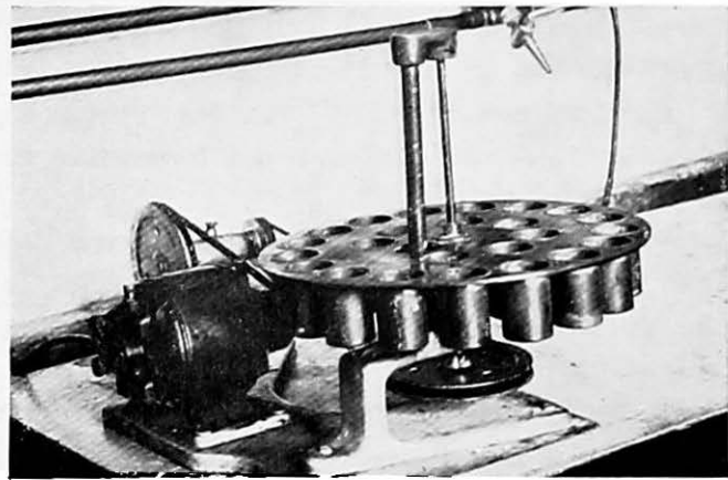
Electrically operated centrifuge, with thermostat, speed indicator, and thermometer. (Fig. 2)
