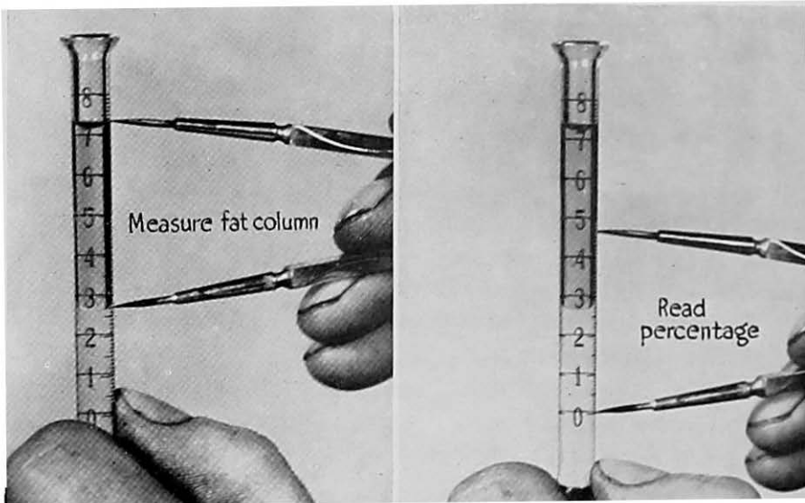
Measuring the fat column. Use sharp-pointed calipers to read the fat column in the test bottle. Place lower pointer at extreme bottom of the fat column and upper pointer at upper edge of meniscus. Then using great care not to change the spread of the calipers, put lower pointer on zero mark. The upper pointer will then point to the fat percentage. Read to nearest tenth of 1 percent. (Fig. 15)
