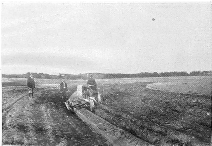
FIGURE 34.—Plowing a channel terrace in order to maintain proper cross section. Note how the channel is being plowed out and how the terrace has been blended into the lower slope.
