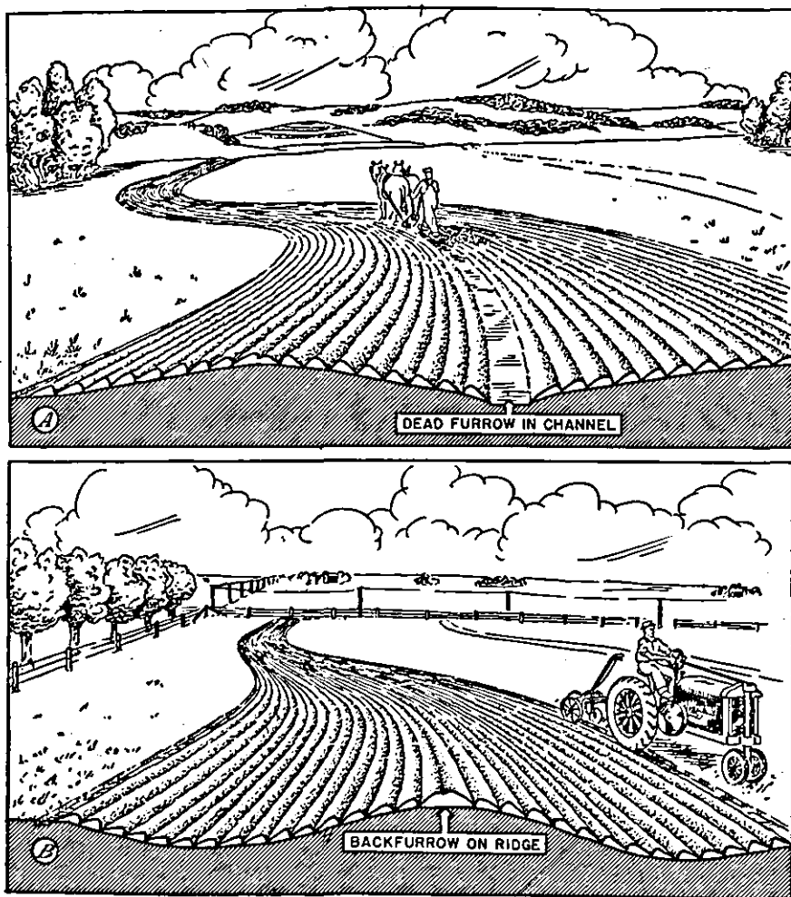
FIGURE 35.—Maintaining terraces by plowing: A, The channel of the channel terrace can be enlarged by plowing it out. Between channels turn as many of the furrows uphill as possible to offset the natural soil movement down the slope. B, The ridge of the ridge terrace can be enlarged by backfurlowing to it. The location of the dead furrow should be varied from year to year to avoid excessive depression at any one point.
