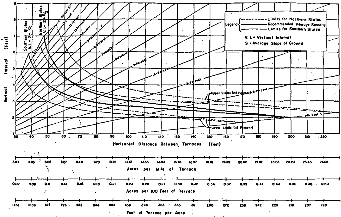
FIGURE 19.—Recommended terrace spacings and related data for channel terraces.
