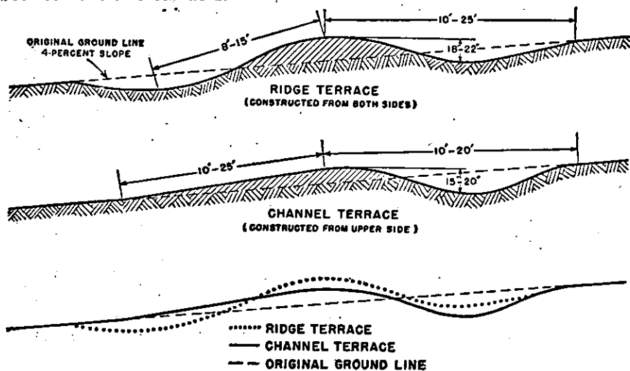
FIGURE 7.—Terrace cross sections after settlement and cultivation.
