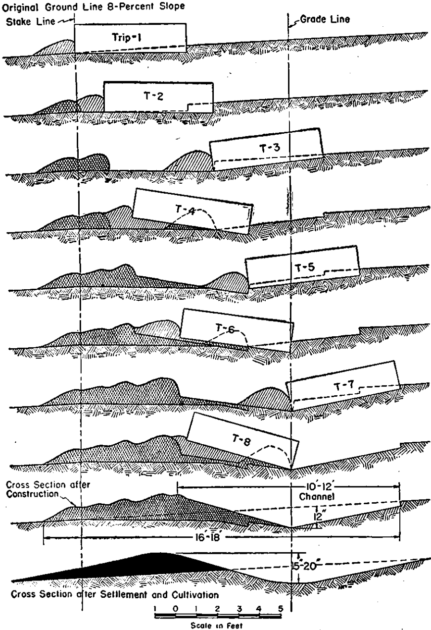
FIGURE 28.—Progressive steps in constructing a channel terrace in the South-east with a 10-foot blade terracer. The terrace is constructed from the upper side only.
