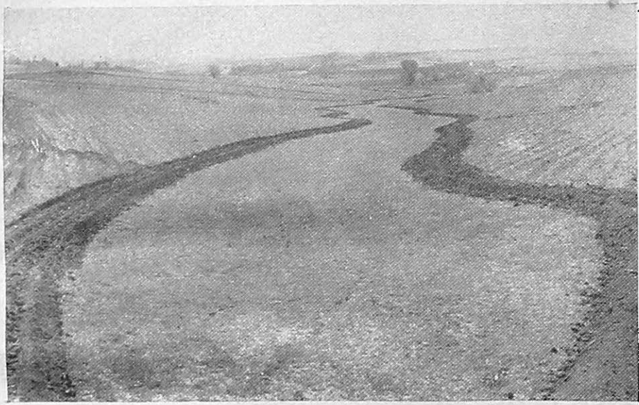
FIGURE 15.—Ridges along the sides protect newly seeded meadow outlet. Terraces will be constructed when the sod is well established.
