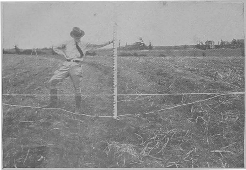
FIGURE 8. —A channel terrace in the Piedmont area. It is important that a wide channel with ample capacity be provided.
