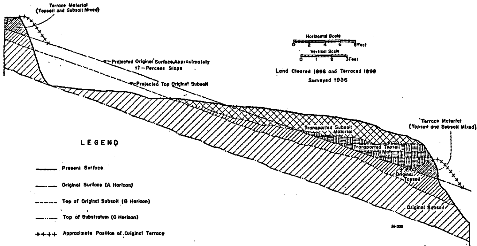
FIGURE 13.—Cross section of a bench terrace. The inverted soil profile has been developed by soil movement between terraces. Unless the topsoil is relatively deep in comparison with the vertical interval between terraces, subsoil is eventually exposed over the entire surface.
