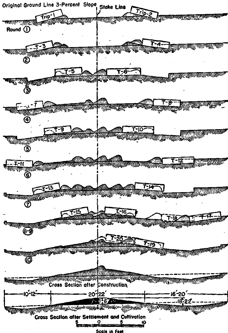
FIGURE 27.—Progressive steps in constructing a ridge terrace in the Great Plains with a 10-foot blade terracer. The terrace is constructed from both sides. With inexperienced operators and on certain soils it may be desirable to secure the necessary center height during the first few rounds.
