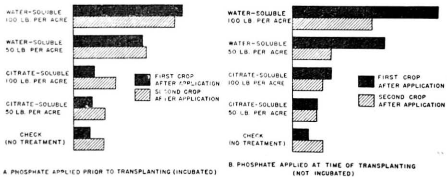
Figure 9.—These are comparative dry-weight yields of Romaine lettuce plants receiving different types and treatments of phosphate fertilizer. Plants were 4 weeks old (from seedling) when they were transplanted. No significant difference in results was obtained between the 30-, 60-, and 90-day incubation; therefore, these were averaged in "A". There was a difference in yield between the incubated soil and non-incubated soil as is shown by a comparison of "A" and "B". Yield responses in these greenhouse tests on high-lime soils were greater from water-soluble phosphate than from citrate-soluble phosphate.
