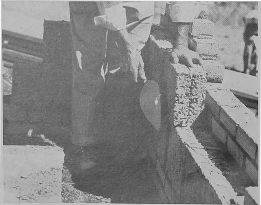
Figure 3.—Insulating block of wood-waste concrete being laid in wall. Outside wall is brick veneer; inside finish may be plaster applied directly to block.
