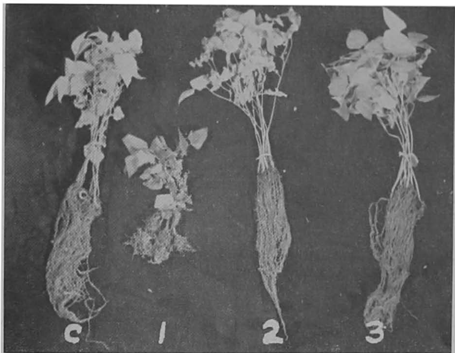
Figure 12.—Effect of ammonium 2,4-D on root growth of beans (typical of the legumes tested). Treatments, in pounds per acre, were as follows: (c) none; (1) 0.2 lb.; (2) 0.03 lb.; and (3) 0.003 lb.
