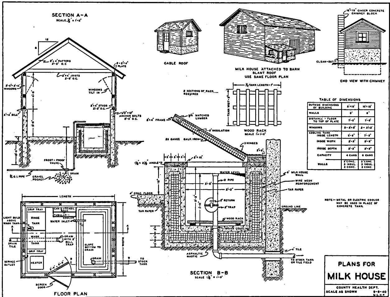
Figure 5. Plan and detail for milk house and cooling tank construction
