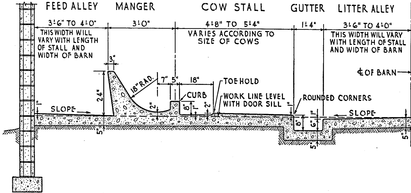
Figure 19. Cross section of a typical dairy barn floor. Dimensions will vary depending upon width of barn
