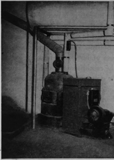
Figure 50. Small coal stoker with insulated storage tank suitable for supplying 170° F. water for the small restaurant
