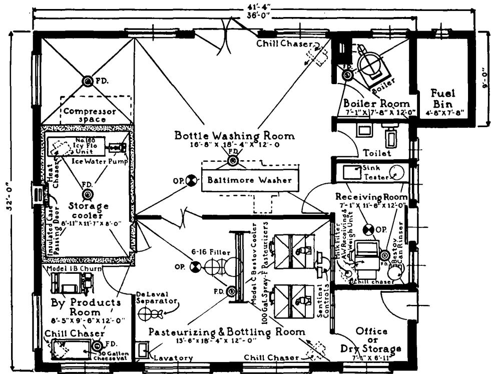
Figure 21. Plan for a small milk pasteurization plant
