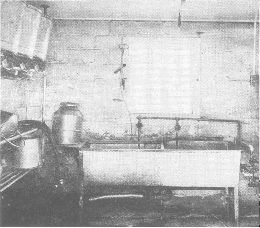
Figure 8. Two-compartment utensil-washing vat of a type suitable for the plant producer
