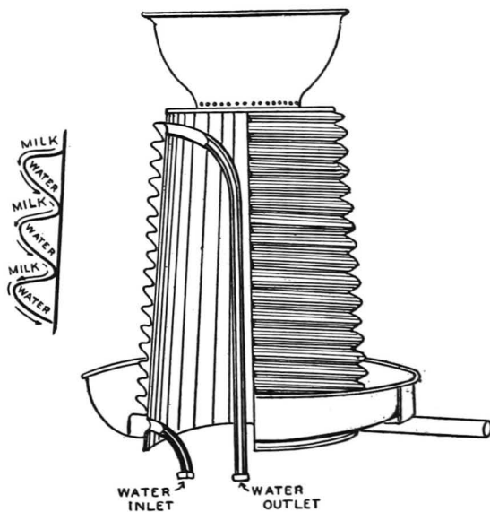
Figure 12. Spiral corrugated milk cooler. Cold water circulates on the inside; milk runs over the outside to be cooled
