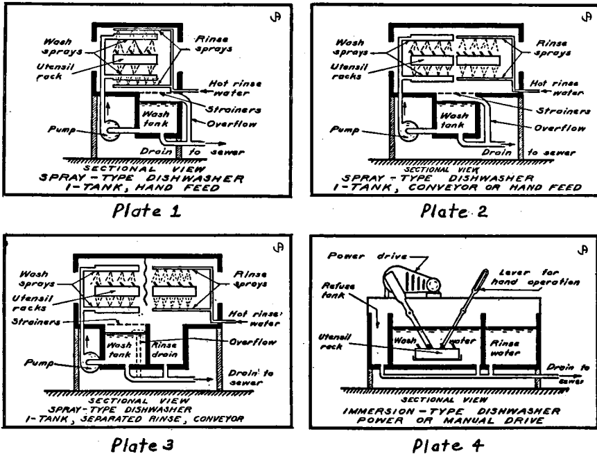
Figure 48. Sectional views of several types of dishwashing machines
