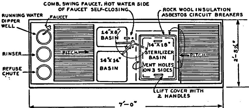
Figure 44. Plan view of glass-washing and sanitizing arrangement suitable for use at a fountain or lunch counter. Note sanitizing vat on right which permits immersion of baskets of glasses in water at 170° F. or above
