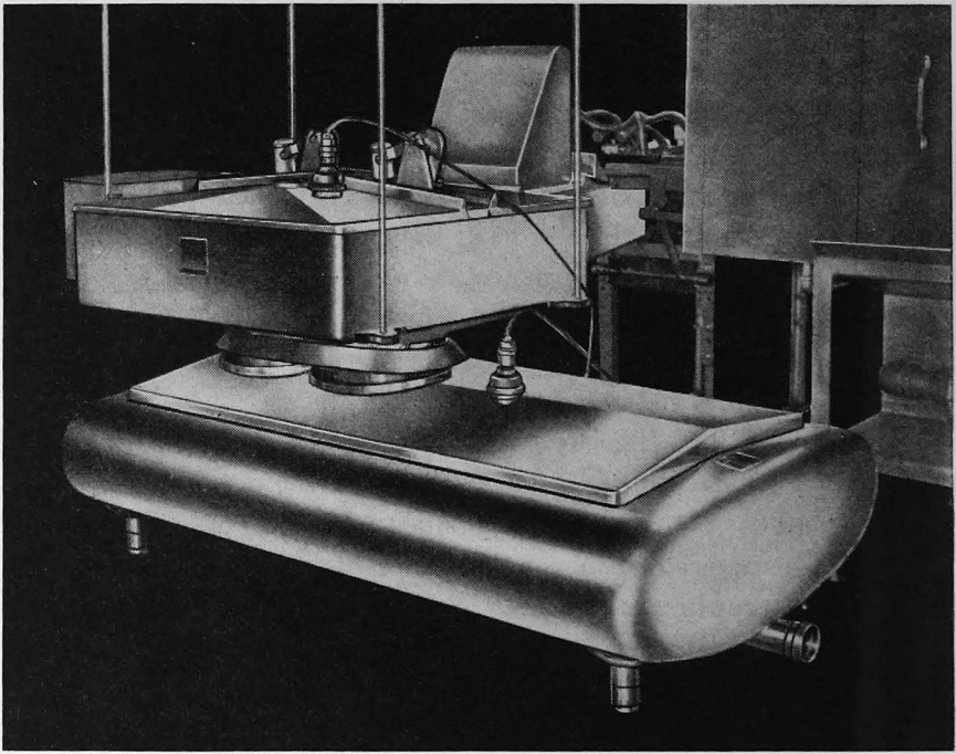
Figure 23. Standard stainless steel weigh and dump tank assembly
