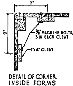
Figure 15. Plan for the construction of an insulated milk-cooling tank
