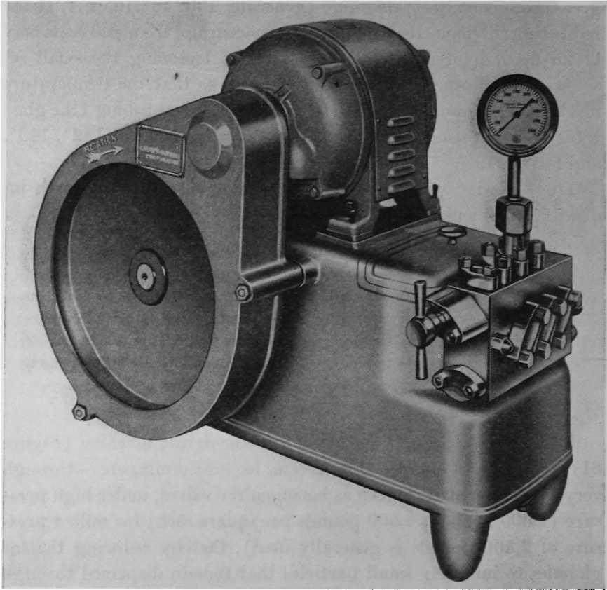
Figure 31. Modern homogenizer, so constructed that milk contact parts can be disassembled for cleaning
