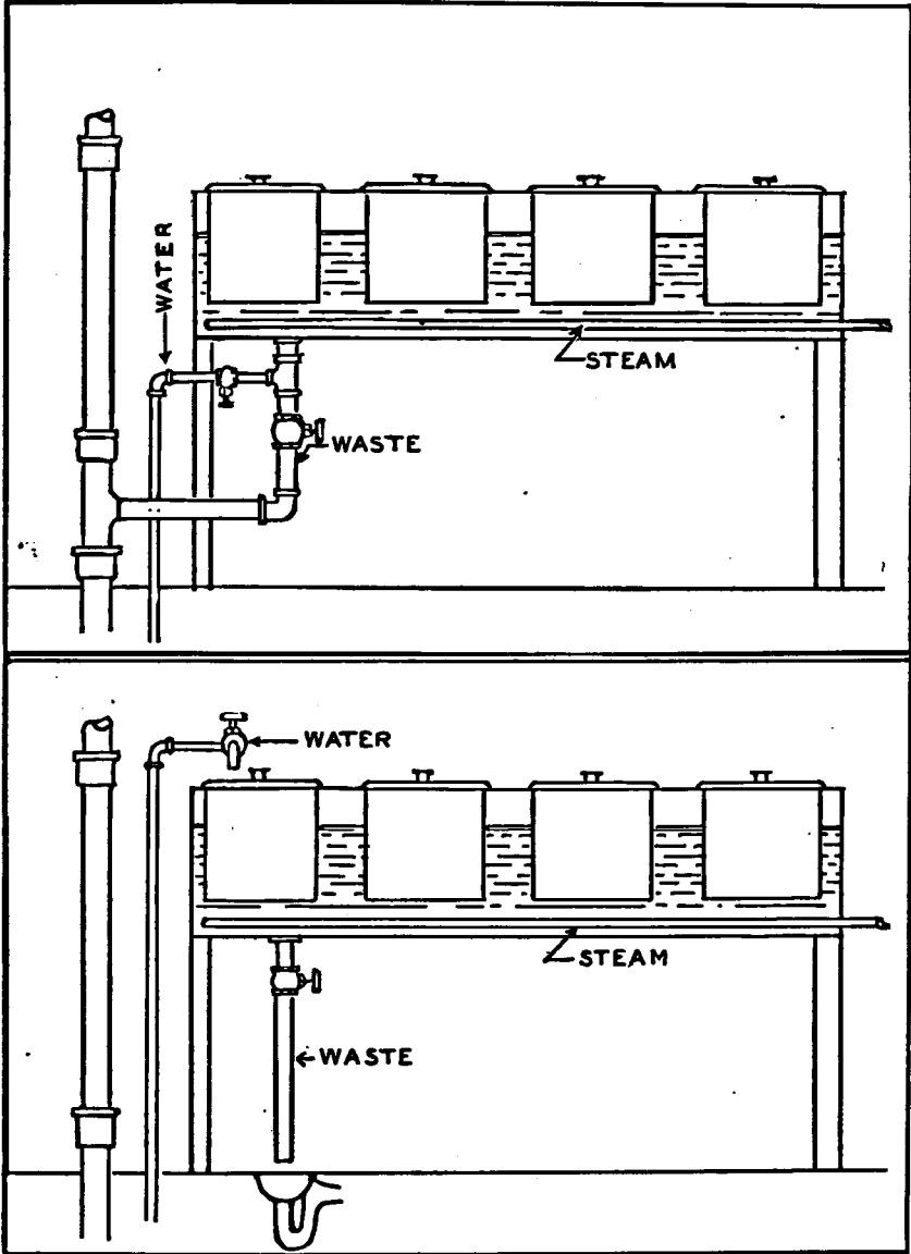
Figure 35. Steam table installations: top, insanitary, with submerged water inlet; bottom, satisfactory installation
