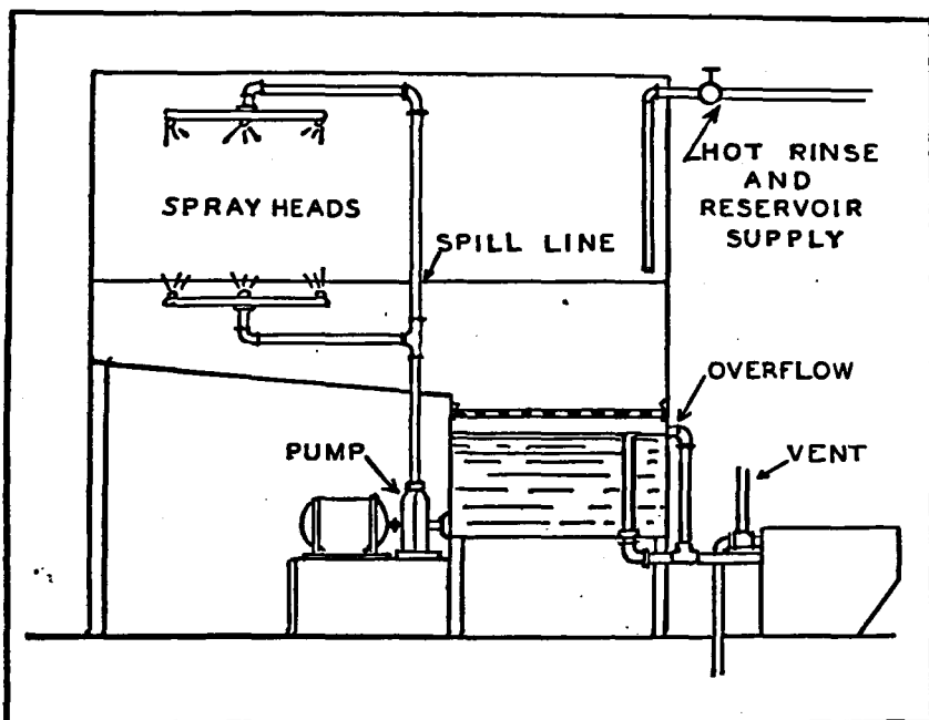
Figure 37. Sanitary dishwashing machine installation
