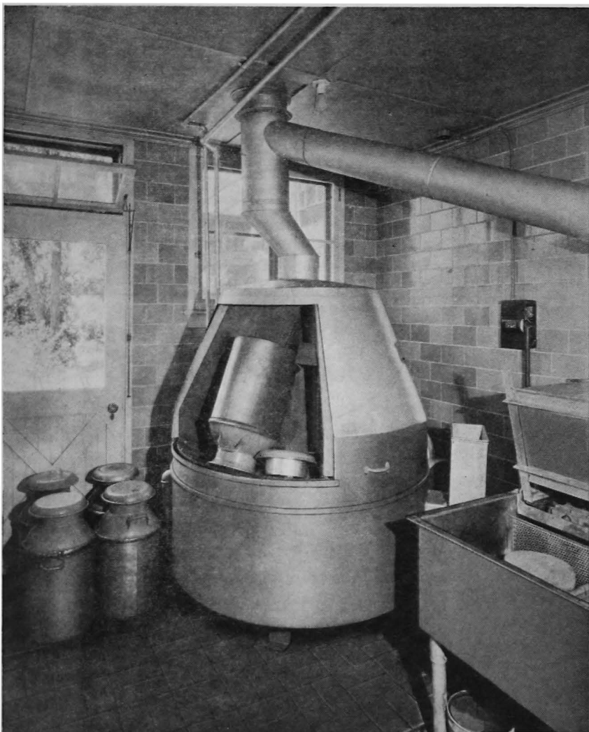
Figure 24. Rotary can-washer installation commonly used in the milk plant
