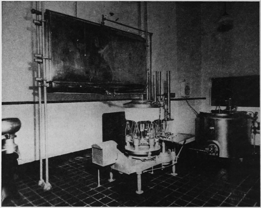
Figure 32. A covered milk cooler is essential for protecting pasteurized milk from contamination
