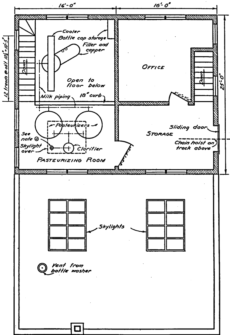
Figure 22b. Plan for a medium-sized pasteurization plant—Mezzanine floor
