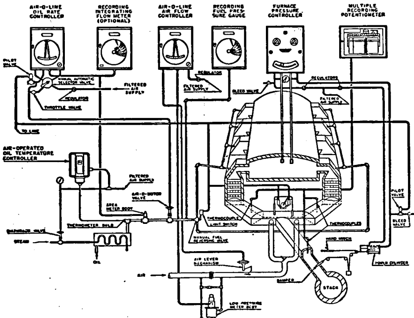
FIG. 16.—Automatic control of an oil-fired glass-melting furnace.
