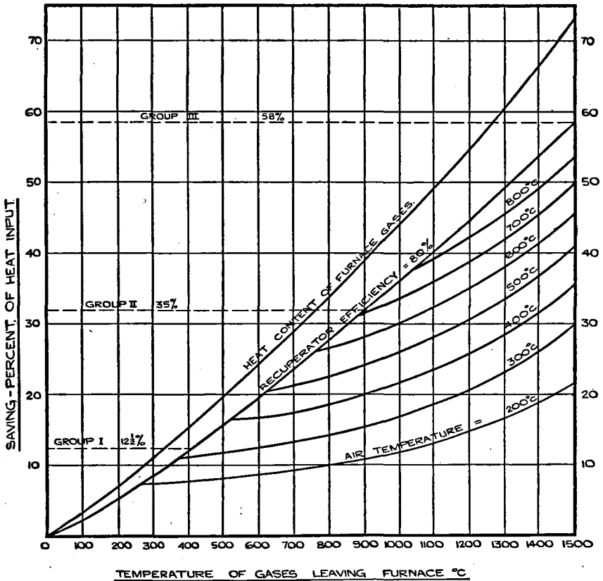
Fig. 24.—Possible Saving by Recuperation of the Combustion Air, for Coke-Oven Gas.
