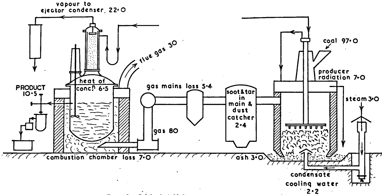
FIG. 25b. Sulphuric Acid Concentration—Producer Gas Firing.
