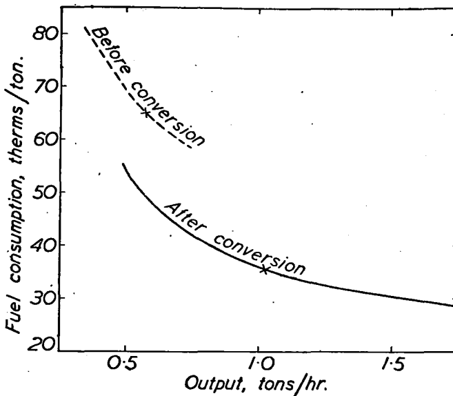
FIG. 7.—Heat Consumption—Output Chart.
