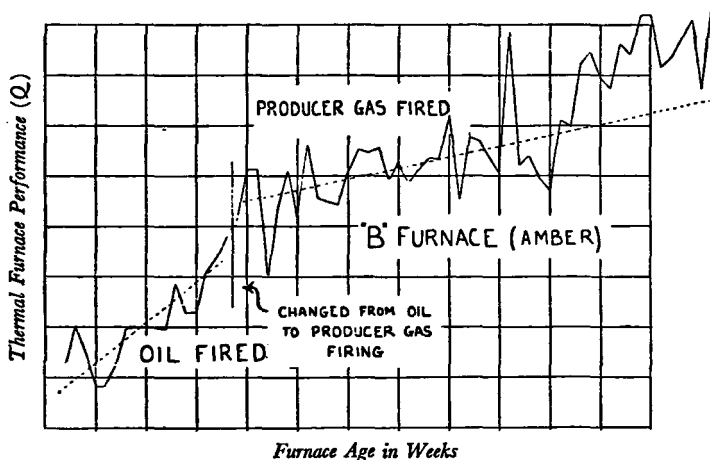
FIG. 19.—The "aging" of a tank furnace when heated by producer gas and oil respectively.
