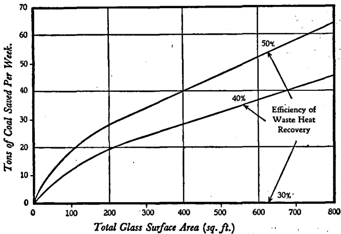
FIG. 15.—Relationship between efficiency of heat return and tons of coal saved per week.
