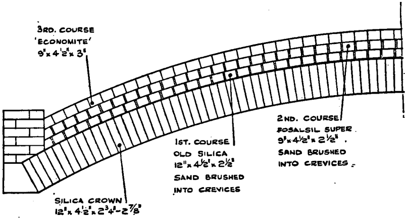
FIG. 12.—Application of insulation to furnace crown.
