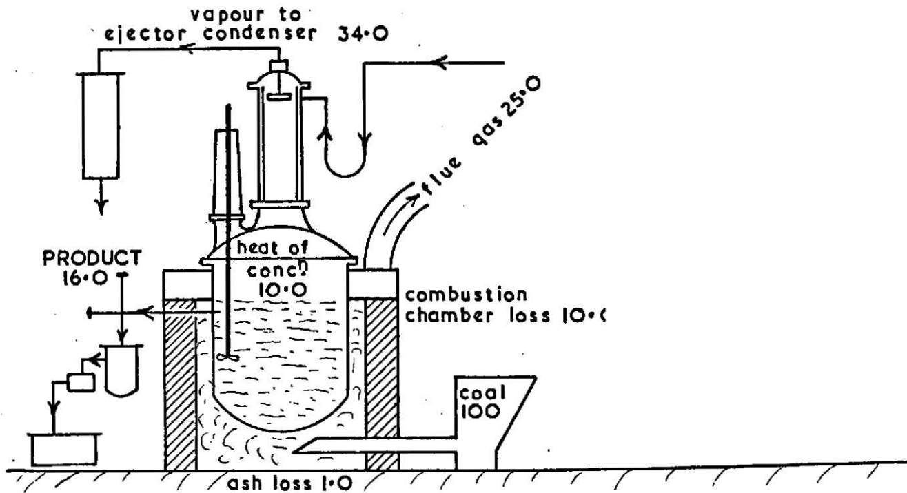
FIG. 25a. Sulphuric Acid Concentration—Direct Firing by Underfeed Stoker.
