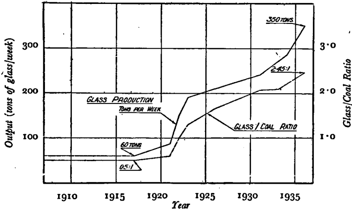
Fig. 9.—Increase in output of a tank furnace melting bottle glass.
