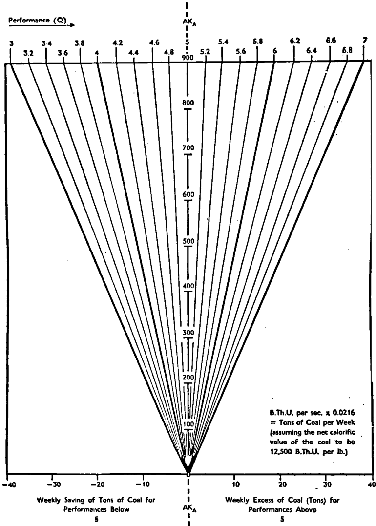
FIG. 18.—Relation between thermal furnace performance and fuel consumption for glass tank furnaces of varying size.
