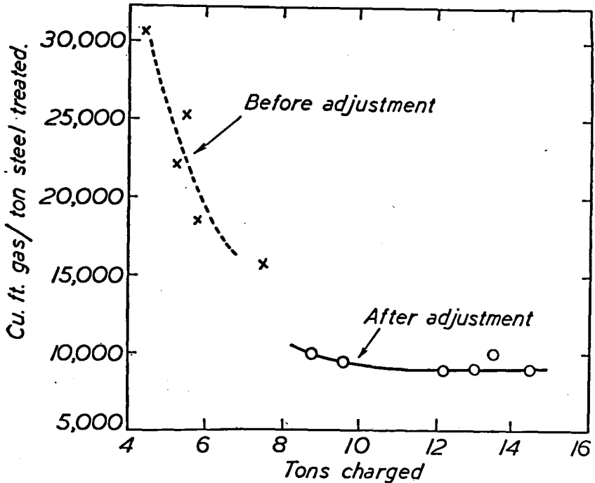
Fig. 6.—Relationship between Fuel Ratio and Weight of Charge for Forced-circulation Heat-treatment Furnace.
