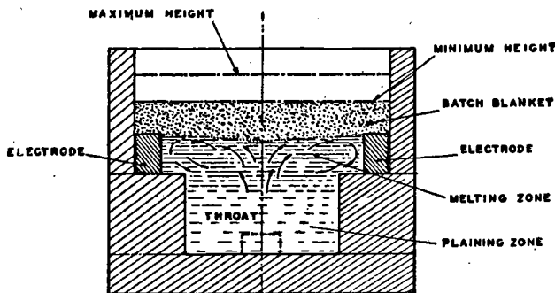
FIG. 10.—Cross-section through electric furnace for melting glass.
