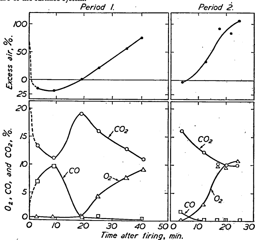
FIG. 1.—Variations in Composition of Furnace Atmosphere of Hand-fired Furnace. (Periods 1 and 2 relate respectively to firing periods during the early and later stages of heating up from cold.)
