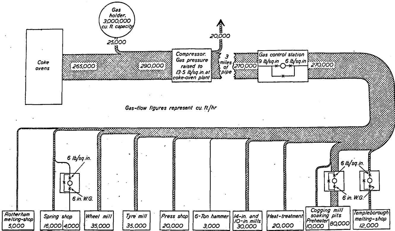
FIG. 8.—Gas Distribution System to Steelworks.
