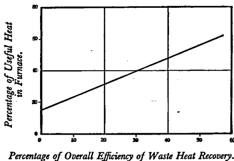
FIG. 14.—Relationship between efficiency of heat return and useful heat in the furnace.
