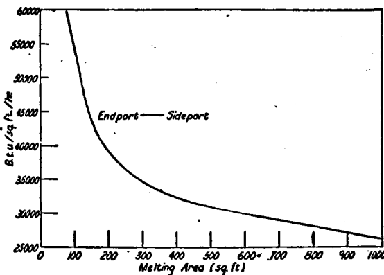
FIG. 11.—Relation between size of melting area and fuel consumption required per sq. ft. of melting area per hour.
