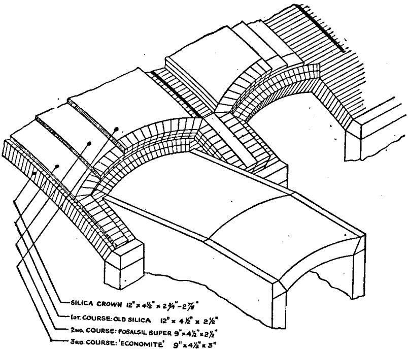
FIG. 13.—Application of insulation to furnace crown.
