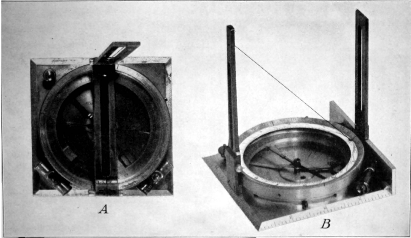
FIGURE 7.—A, Forester's or geologist's compass; B, sundial compass.
