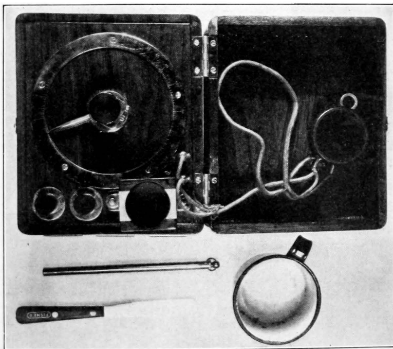
FIGURE 16.—Portable electrolytic bridge, with box open and cup in place ready for use. On the side are shown the mixing cup, spatula, and thermometer.
