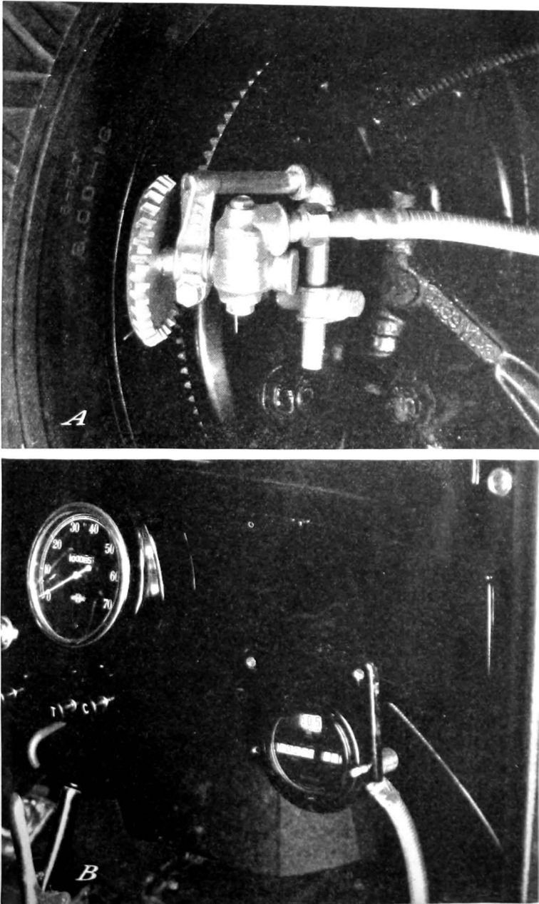
FIGURE 3.—A. Complete assembly in correct position for operation. By loosening the clamps on the end of the stud bolt, the fiber gear may be disengaged while the speedometer is not needed. B. Speedometer head in correct position on the dash.
