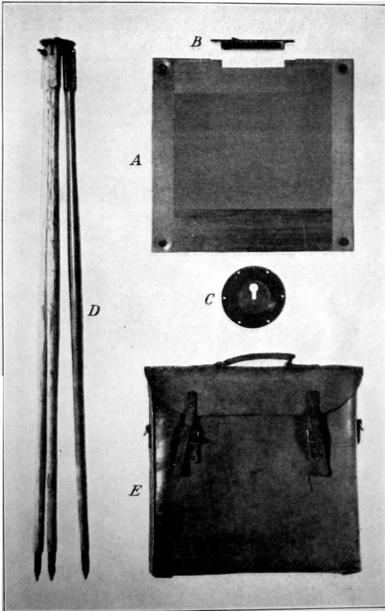
FIGURE 4.—Plane table, unassembled: A , board; B , compass; C , head; D , tripod; and E , case.
