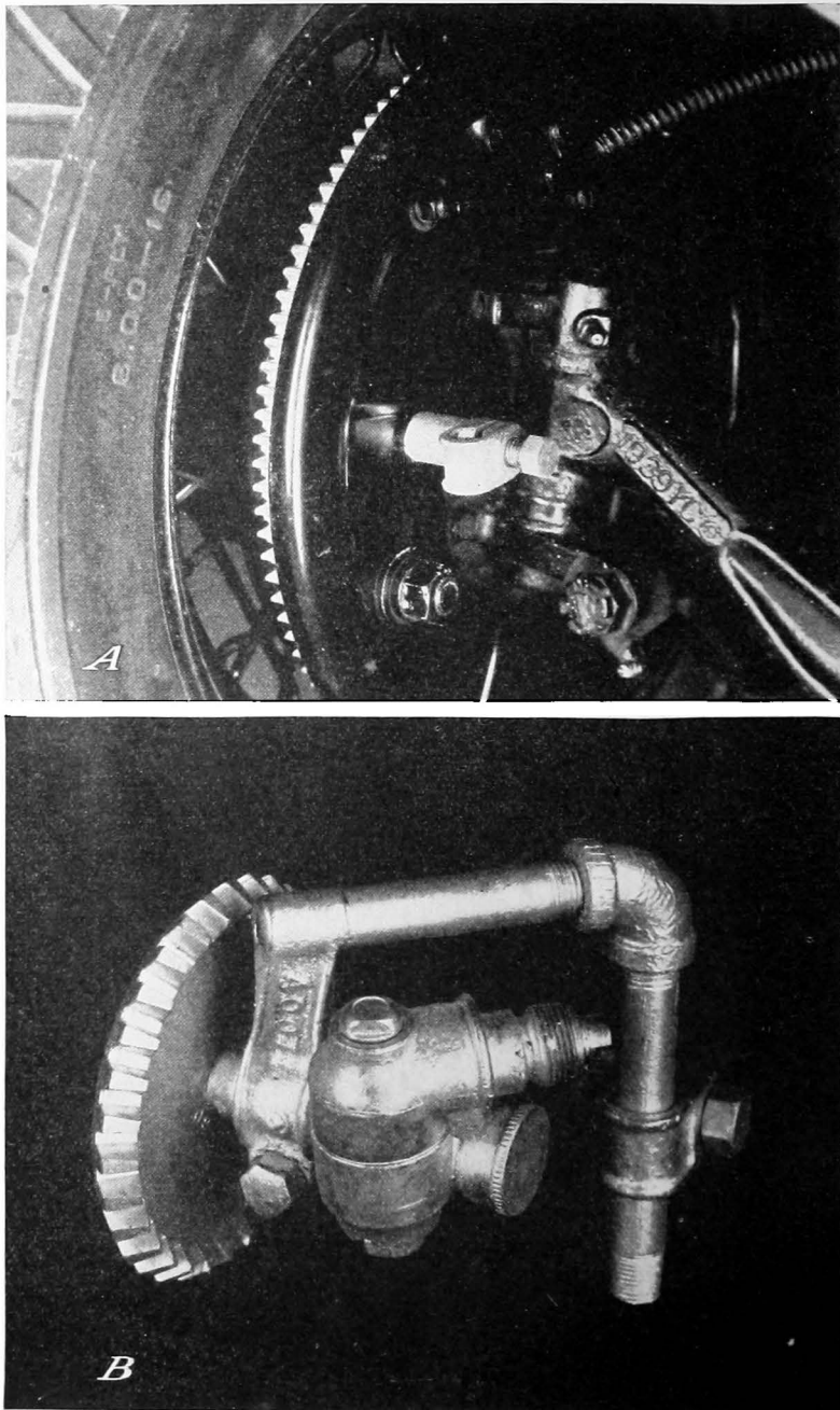
FIGURE 2.—A, The stud bolt in position on the brake housing; B, the assembly for attaching fiber gear after twisting angle bar 4007.
