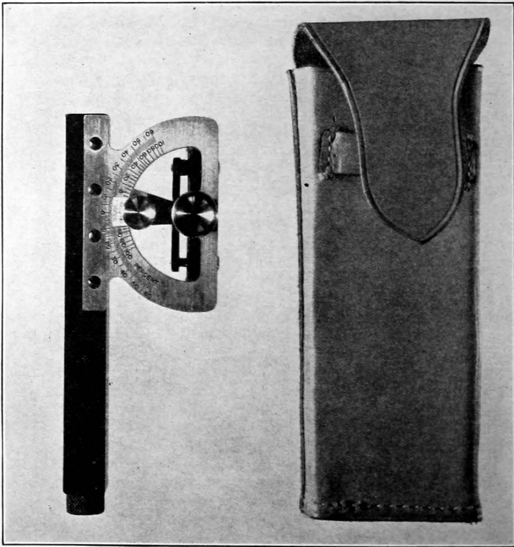
FIGURE 14.—Abney hand level, with case.
