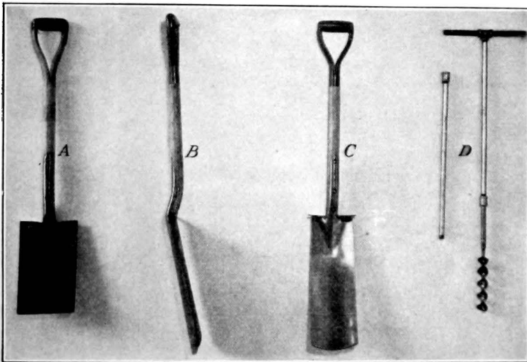
FIGURE 8.—Soil-sampling tools: A , square-pointed spade, especially useful in collecting samples; B , side view and C , front view of post-hole spade, the most generally useful sampling tool; and D , soil auger with extension.
