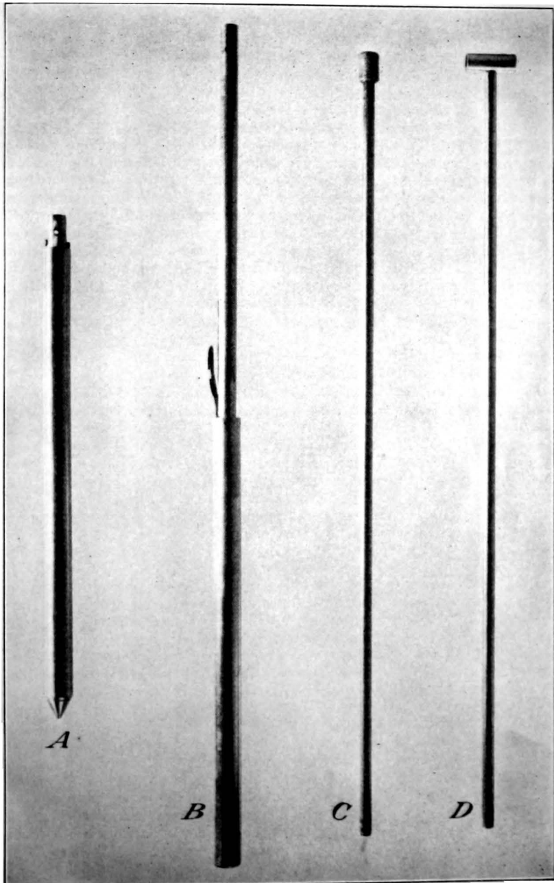
FIGURE 9.—Pent sampler: A , the head closed, ready for pushing into the peat; B , the head extended, as just prior to taking a sample; C , one 2-foot extension rod, and D , the top extension rod.
