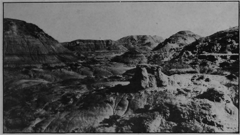
TYPICAL BAD LANDS NEAR HUNGRY CREEK.
