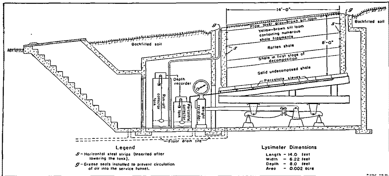
FIGURE 1.—Schematic cross-sectional diagram. A soil-block lysimeter with self-recording weighing mechanism used at the North Appalachian Experimental Watershed, Coshocton, Ohio.
