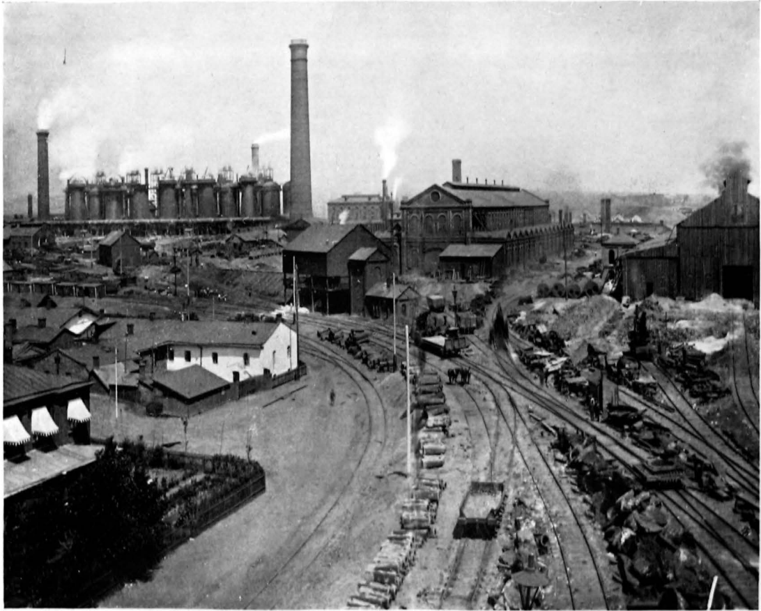
THE NEW RUSSIAN COMPANY'S IRON AND STEEL WORKS, YUZOVO.
