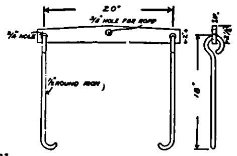
DETAIL OF YOKE AT "E"
