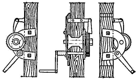
DETAIL OF WINCH AT "D"
