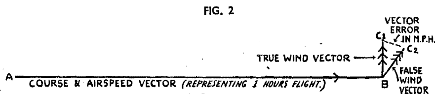
Wind-finding by method of triangle of velocities
