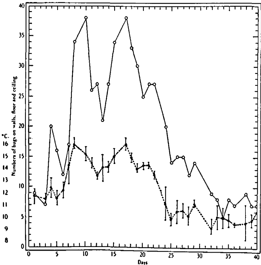
FIG. 7. Correlation of activity in experimental hut. Dotted line represents mean daily temperature; vertical lines indicate mean maximum and mean minimum daily temperatures. Unbroken line: number of bugs daily on walls, floor and roof. (For further details see Johnson, 1941, Tables 46, 52 and 53.)
