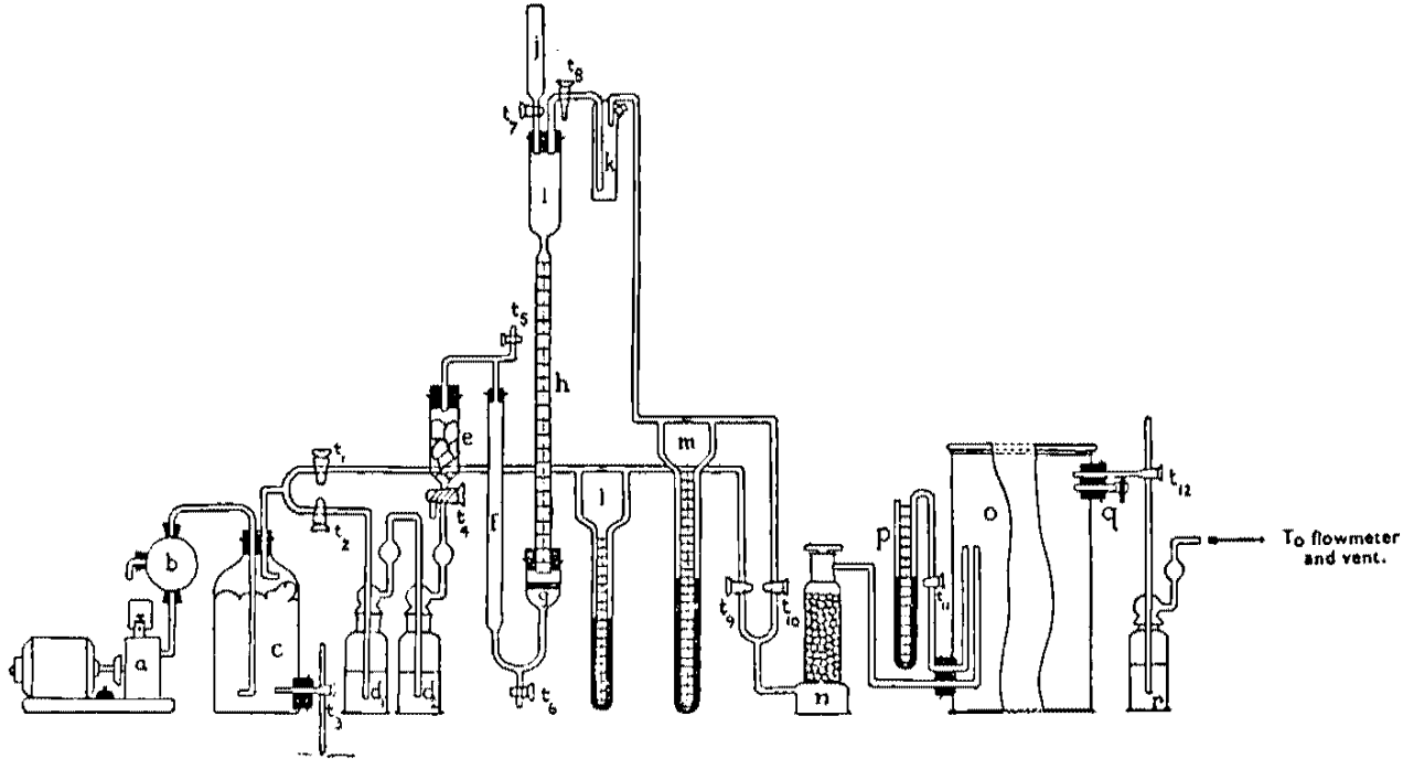
FIG. 9. Apparatus for exposing small animals to methylated benzenes.
