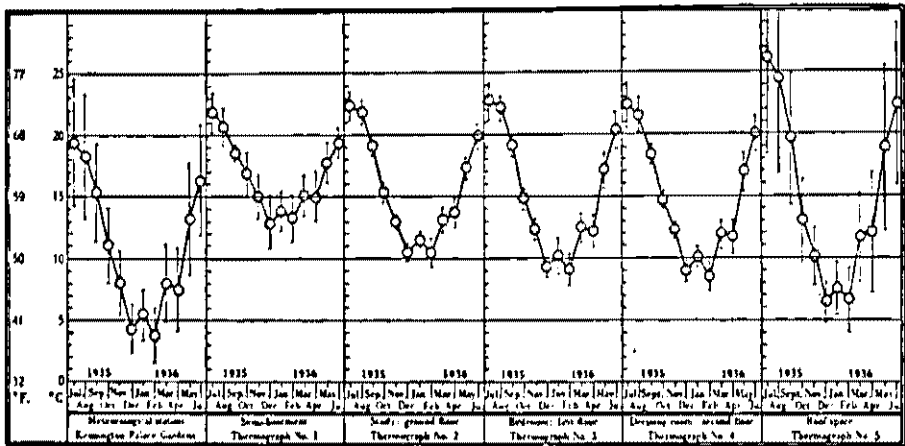
FIG. 2. Mean monthly temperatures, and mean maximum and mean minimum monthly temperatures, in rooms of 54, Palace Gardens Terrace, London, for 1935-6. Circles indicate mean monthly temperatures. Vertical lines through circles indicate mean maximum and mean minimum monthly temperatures.
