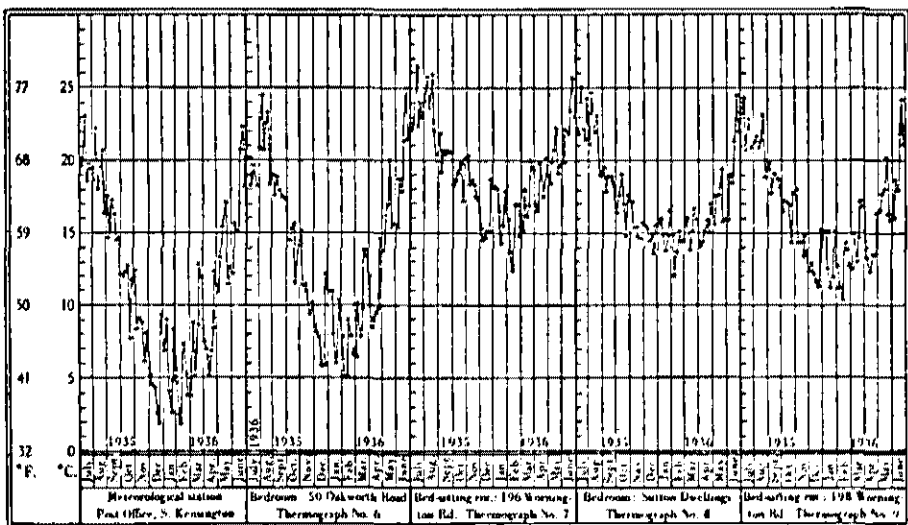
FIG. 1. Temperatures in rooms of various houses in Kensington for 1935-36, expressed as means for 5-day periods.
