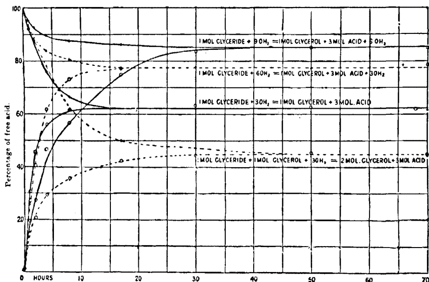
FIG. 2.—Series of Curves Showing the Different Equilibrium Positions of the Oleic Acid-Glycerol Fat-Water System, as Attained Under the Action of Lipase with Different Proportions of Water.
