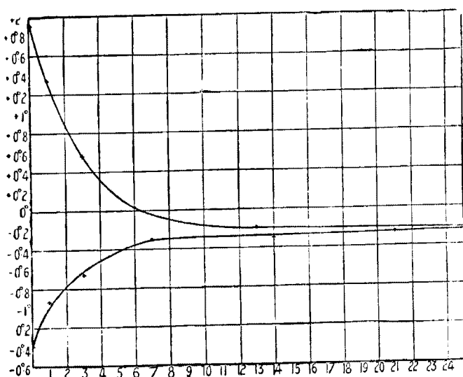
FIG. 6.—Equilibrium Attained Under the Action of Emulsin on Glycerol and Glucose (Upper Curve) and on Glycerol-Glucoside (Lower Curve). The position is the same. Ordinates—optical rotation of diluted samples. Abscissæ—time in days.
