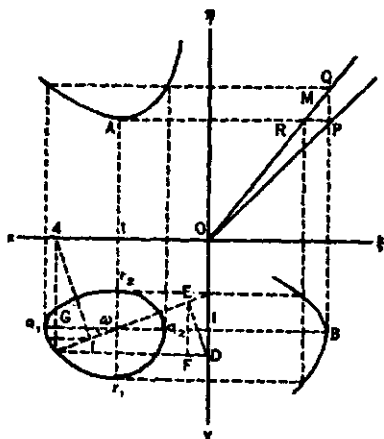
FIGURE 115.—VOLTERRA METHOD OF OBTAINING HYSTERESIS DIAGRAM.
