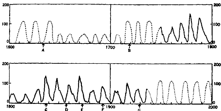
FIGURE 166.—SUNSPOT NUMBERS, 1600-2000 (PARTLY EXTRAPOLATED).
