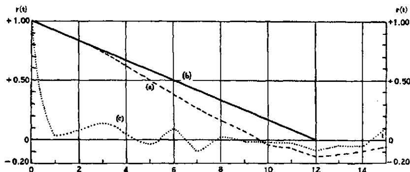
FIGURE 39.—AUTOCORRELATION OF FUNCTIONS.
