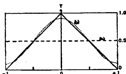
FIGURE 12.—FOURIER APPROXIMATIONS OF CONTINUOUS FUNCTION. (a) First approximation, (b) Second approximation.
