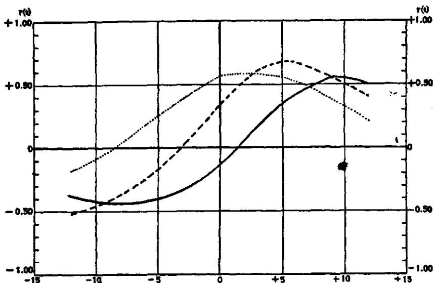
FIGURE 111.—LAG CORRELATIONS.
