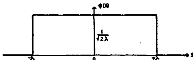
FIGURE 25.—RECTANGULAR FUNCTION.
