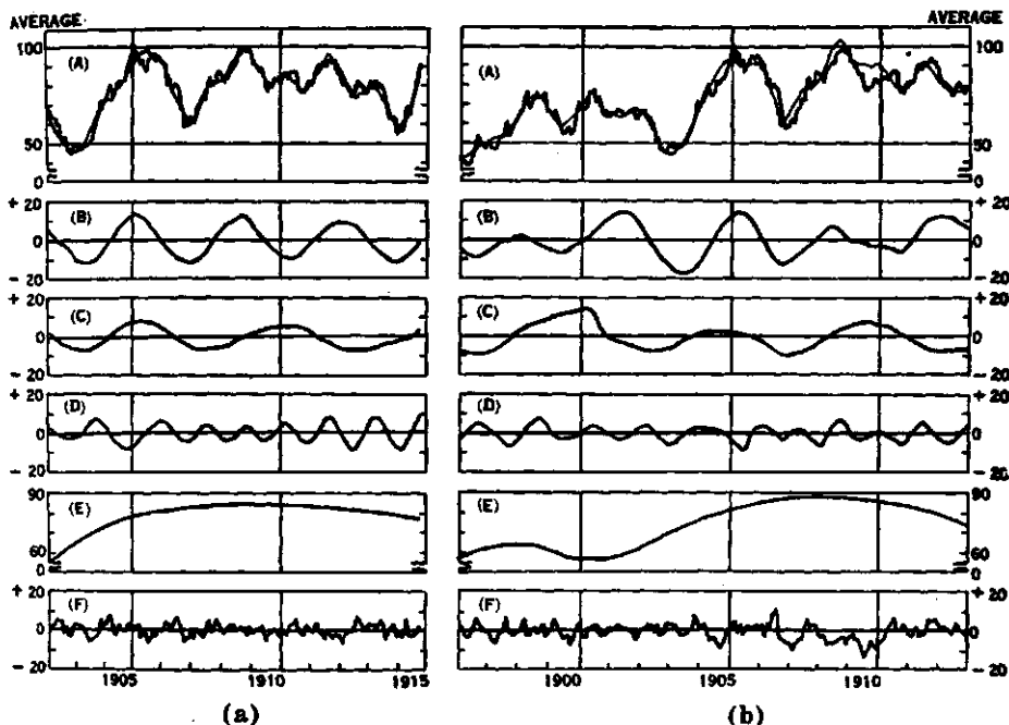
FIGURE 157.—REDUCTION OF TIME SERIES TO RANDOM ELEMENTS.
