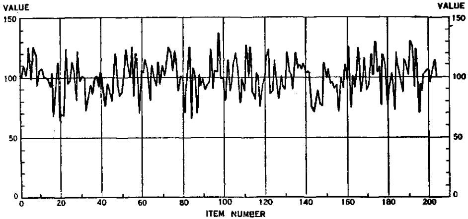
FIGURE 61.—RANDOM SERIES.
