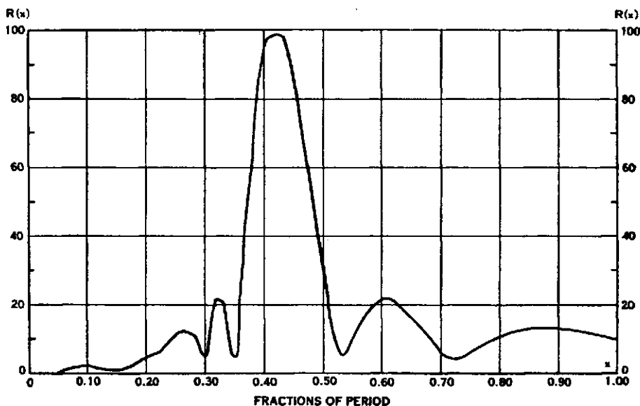
FIGURE 14.—PERIODOGRAM OF SIMPLE HARMONIC.
