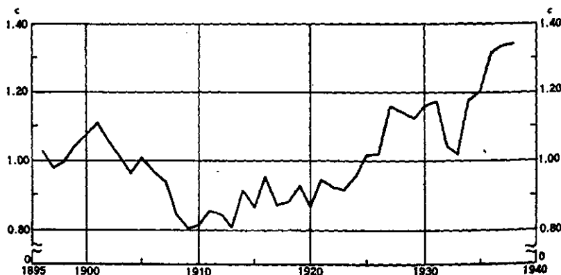
FIGURE 140.—VARIATIONS IN SNYDER'S CONSTANT c . In this chart a constant velocity trend is assumed.
