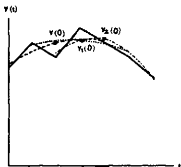
FIGURE 46.—APPLICATION OF SHEPPARD'S SMOOTHING FORMULA.
