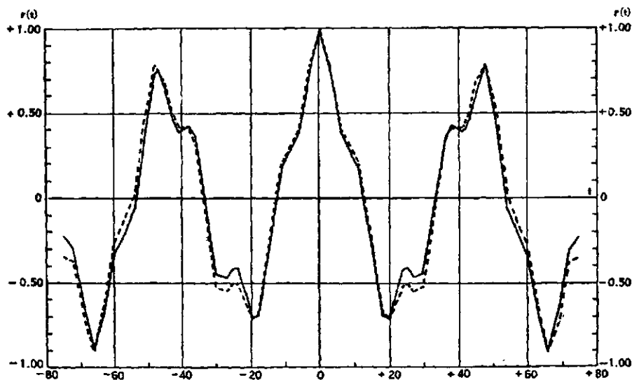
FIGURE 26.—AUTOCORRELATION GRAPH OF A FUNCTION WITH FIVE PERIODIC TERMS. — : r(s) computed by formula; - - - : r(s) computed directly from data.
