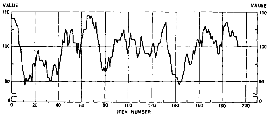
FIGURE 63.—SMOOTHED RANDOM SERIES.
