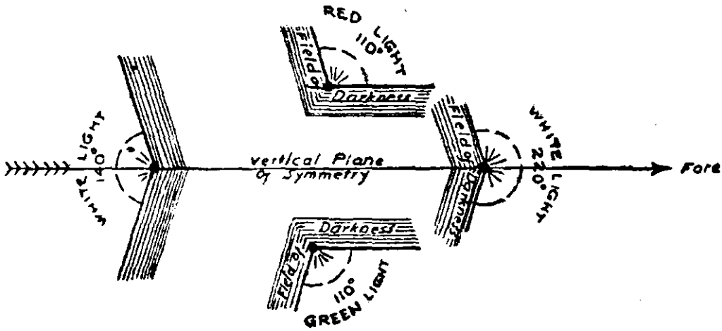
Figure 1. Navigation Lights.—Angular limits prescribed in rule 89.
