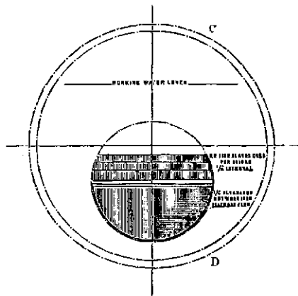
SMOKE-CONSUMING APPARATUS AS APPLIED TO A (ONE-FLUED) CORNISH BOILER.
