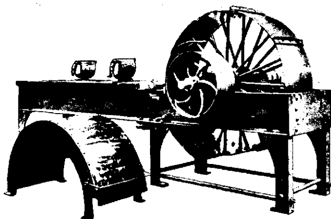
SCUTCHING MACHINE
