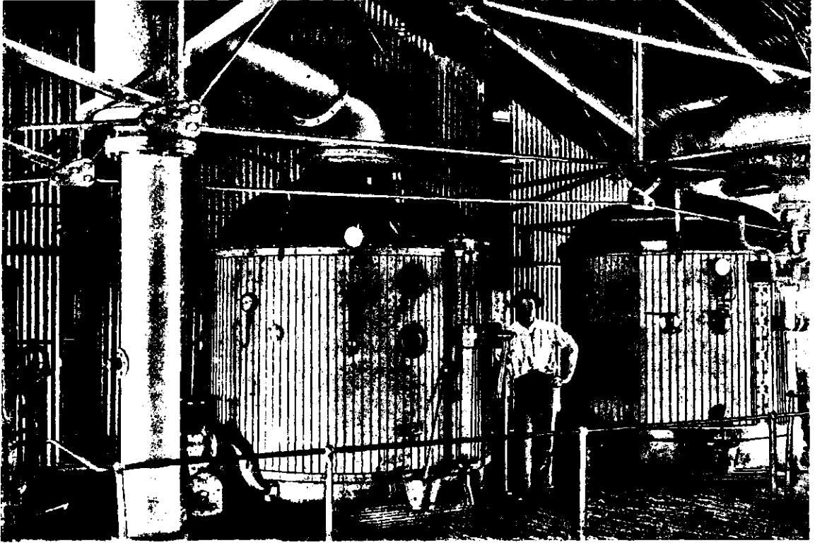
VACUUM PANS
