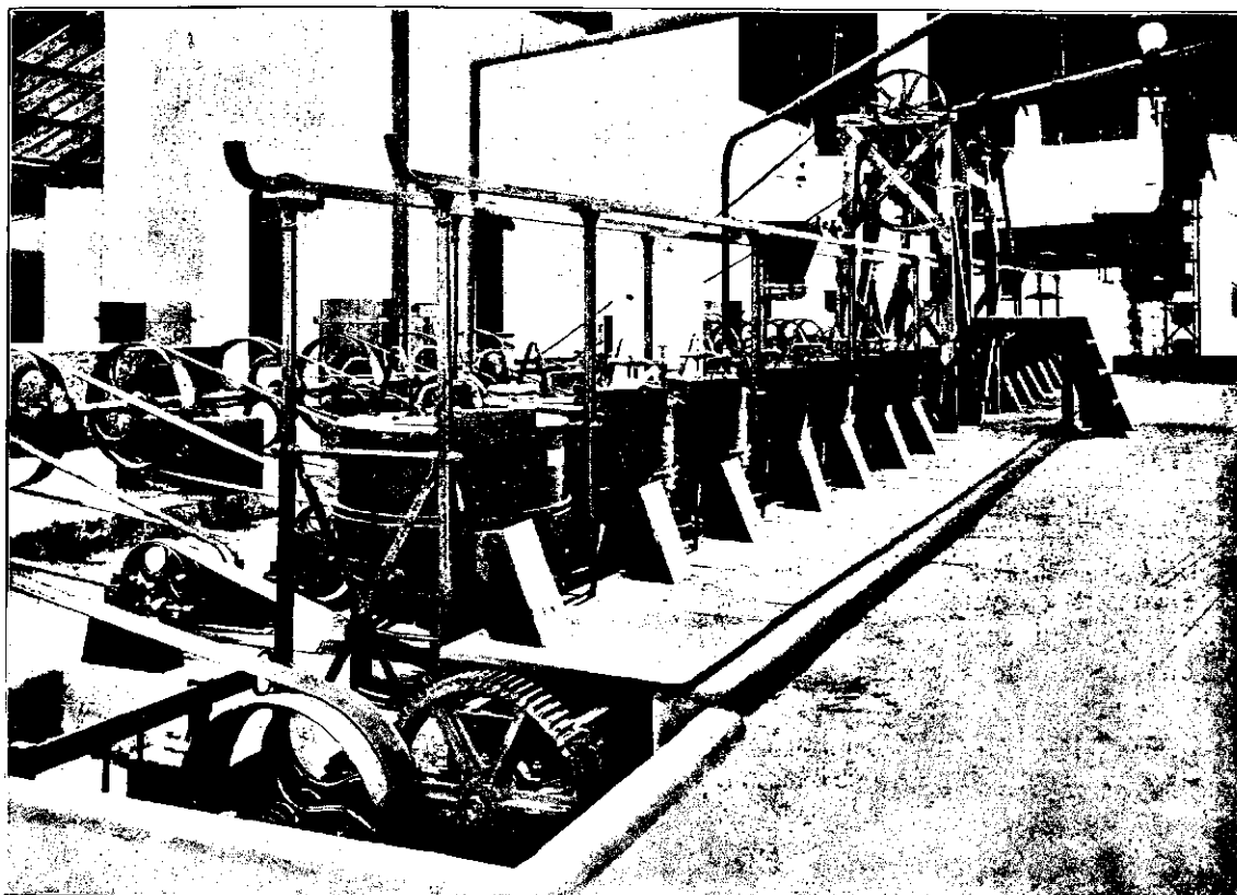
A ROW OF CENTRIFUGAL MACHINES FOR SEPARATING SUGAR CRYSTALS FROM MOLASSES
