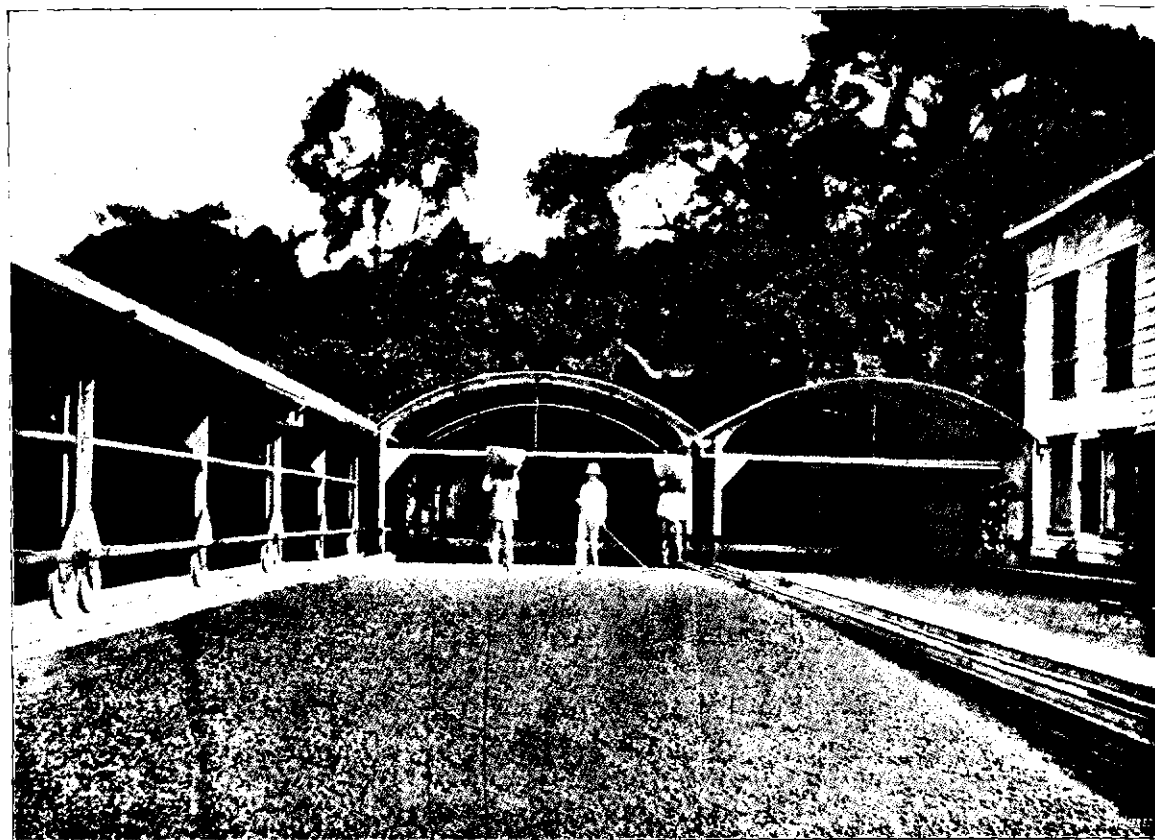
STONE DRYING FLOOR WITH MOVEABLE ROOF
