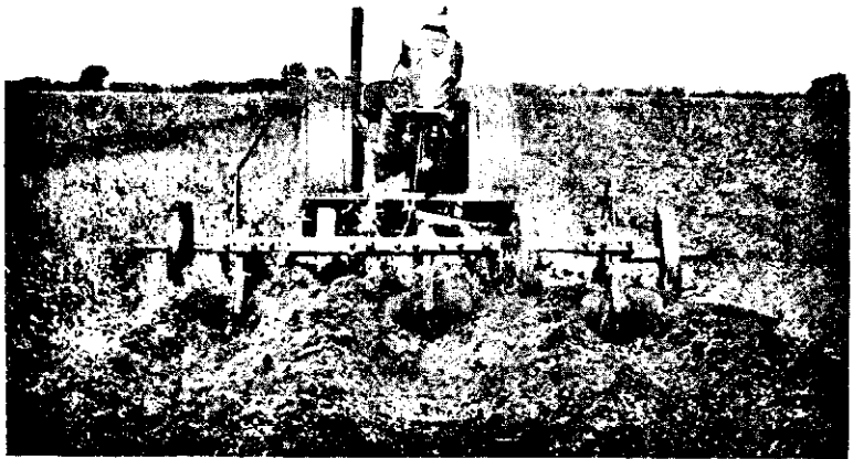
FIG. 143. The lister. Note the depth of furrows produced and the cloddy rather than pulverized condition of the soil. This favors control of erosion. (Courtesy of Deere and Company, Moline, Ill.)
