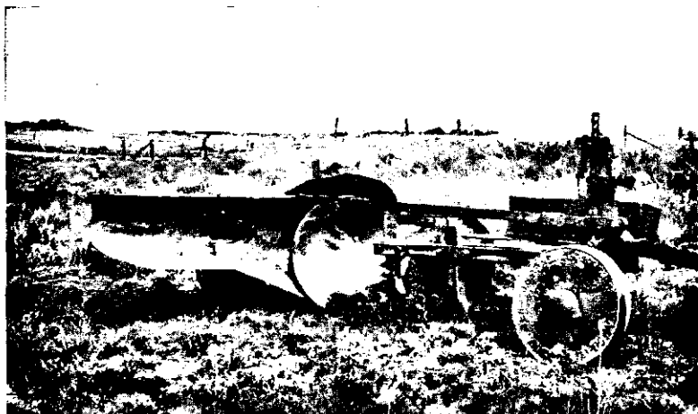
FIG. 105.—Contour-furrowing machine in use in Colorado. An extension moldboard on a disk plow moves the furrow-slice soil several inches over from the edge of the furrow. The soil thrown out of the furrow forms a low dike which increases the capacity of the furrow. (Courtesy of U. S. Soil Conservation Service, Colorado.)
