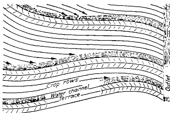
FIG. 99.—Cropping terraces of irregular widths. II. By seeding parallel to the lower side of a terrace ridge, the point rows end in the terrace channel, a very desirable arrangement. (Adapted from North Carolina Agr. Ext. Circ. 173 , by A. T. Holman, p. 13, 1935.)
