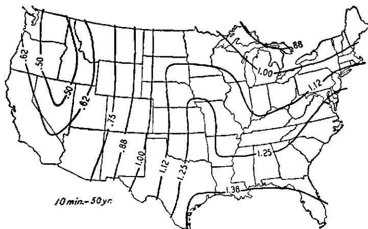
FIG. 27. - Rainfall in inches to be expected in 10 minutes once in 50 years.
