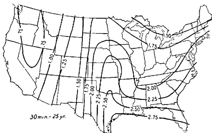
FIG. 28.- Rainfall in inches to be expected in 30 minutes once in 25 years.
