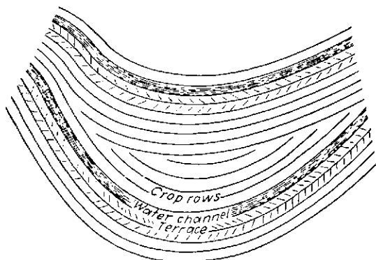
FIG. 98.—Cropping terraces of irregular widths. I. In case of any slope in the rows some washing may take place at the ends of rows in the middle of the terrace. (Adapted from Missouri Agr. Ext. Circ. 317 , by G. E. Martin, p. 18, 1935.)
