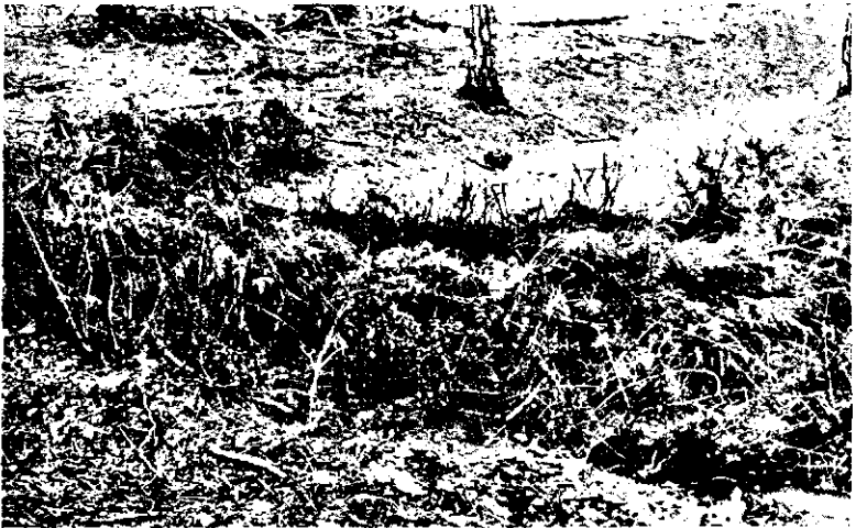
FIG. 89.—Coralberry improves outlet protection. Coralberry ( Symphoricarpos orbiculatus ) was planted in this terrace outlet. This shrub is a distinct aid in the stabilization of this terrace outlet. (Courtesy of U. S. Soil Conservation Service, North Carolina.)
