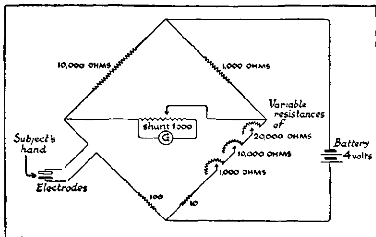
FIG. 62.—Diagram of psychogalvanometer circuit.
