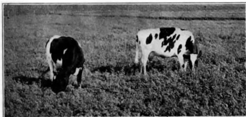
FIG. 5.—INCREASED NITROGEN CONTENT IS AN ALMOST UNIVERSAL NEED OF THE SOILS OF AREA 7
