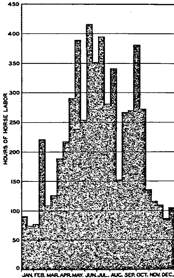
FIG. 11.—SEASONAL DISTRIBUTION OF HORSE LABOR ON A 172-ACRE CLINTON COUNTY FARM
