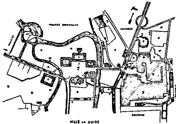
Fig 1. GENERAL PLAN.
