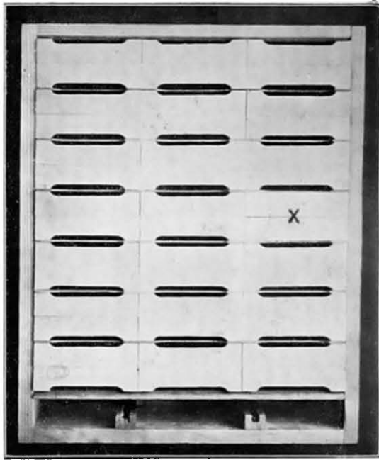
FIG. 36.—ECONOMIC CRATE FILLED WITH "D" SECTIONS.
