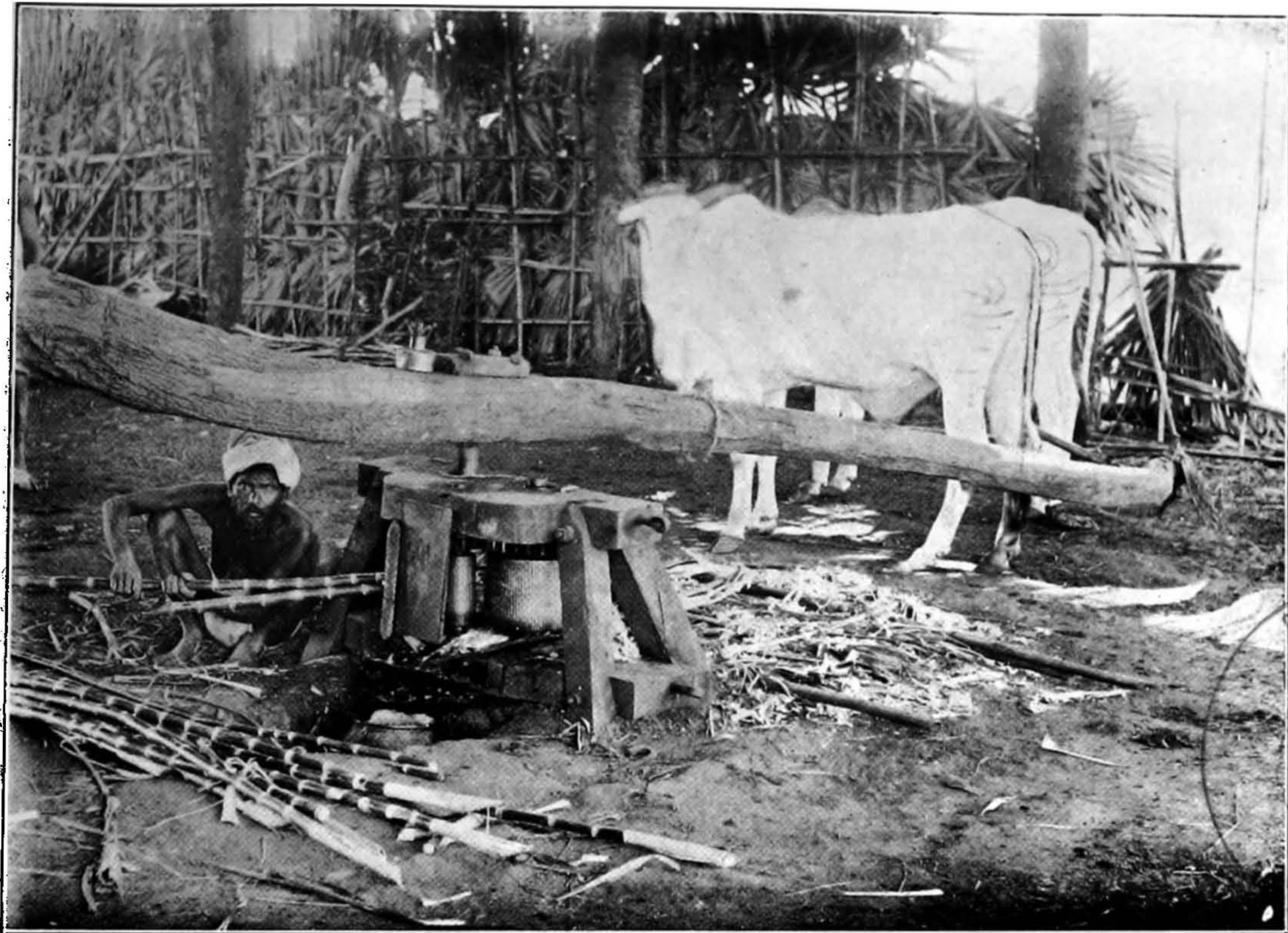
SUGAR-CANE CRUSHING.
