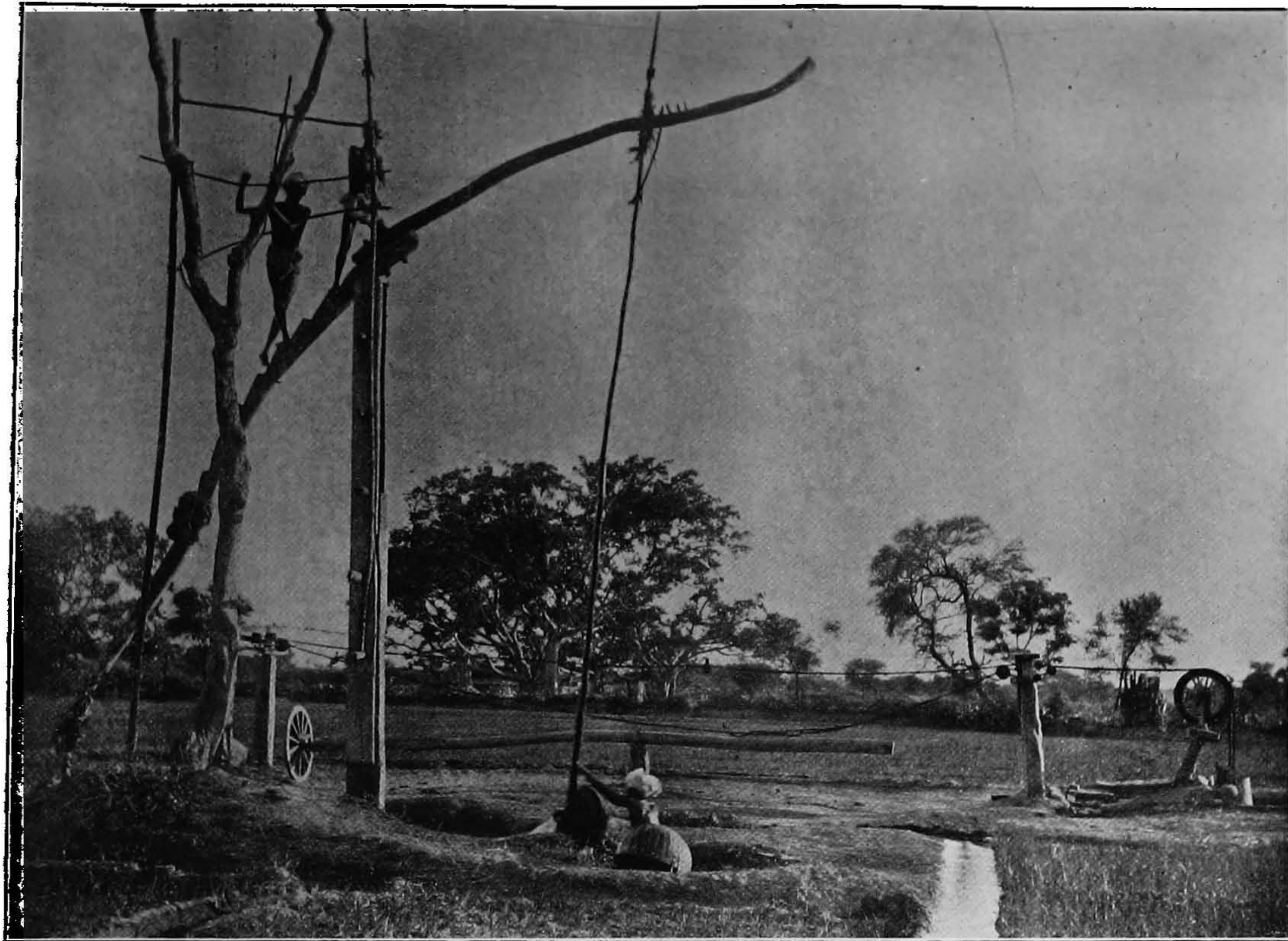
PICOTTAK AND IMPROVED BULLOCK LIFT, USED IN SOUTH ARCOT.
