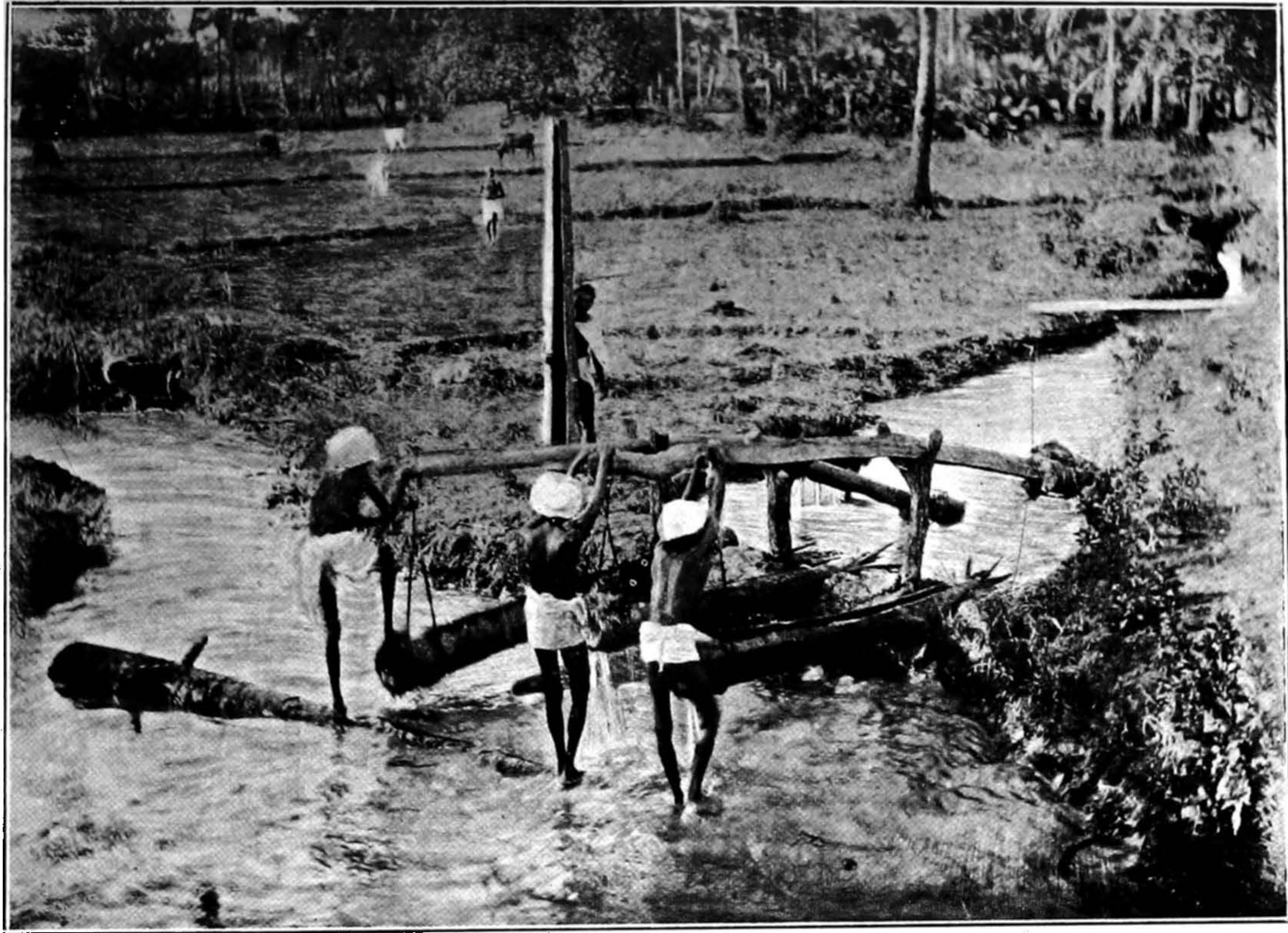
“KARIM”, WATER-LIFT USED IN GODAVARI DELTA. Photo by Agricultural College.
