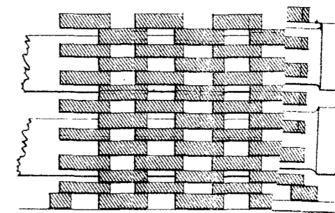
PORTION OF OPEN BRICKWORK SHOWING PIPES 5/8 INCH TO A FOOT
