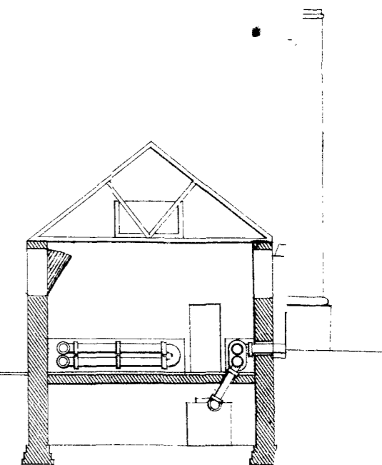
SECTION THROUGH DRYING ROOM
