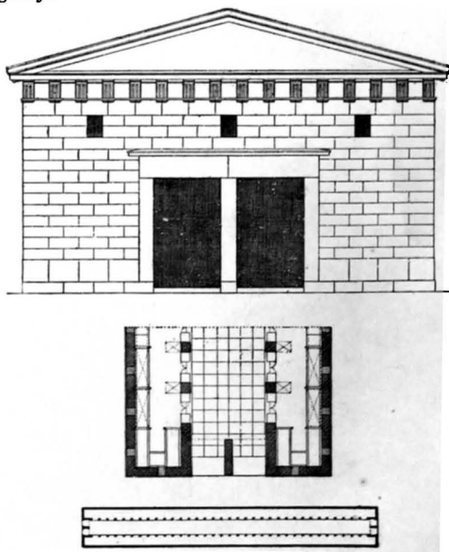
RESTORED ELEVATION AND PLAN OF THE ARSENAL OF PHILON AT PEIRÆUS. 2
