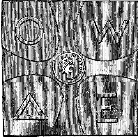
PUBLIC WEIGHTS. 1
