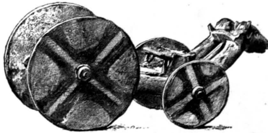
GREEK CART. 2
