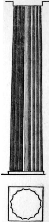
Fig. 56.—DORIC PILLAR AND SECTION OF BASE.—See Page 103.
