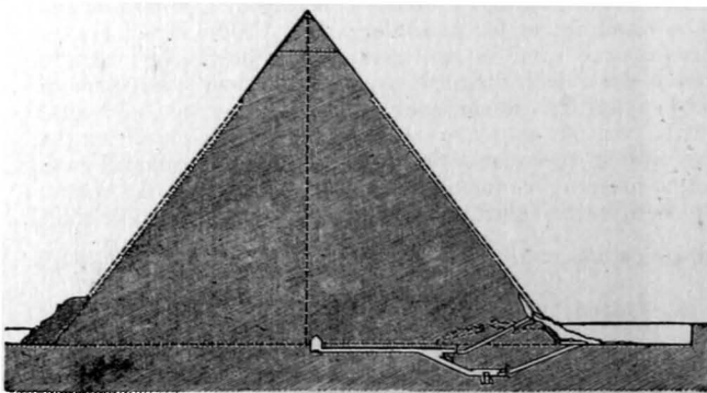
Fig. 46.—SECTION OF THE SECOND PYRAMID.—See Page 96.
