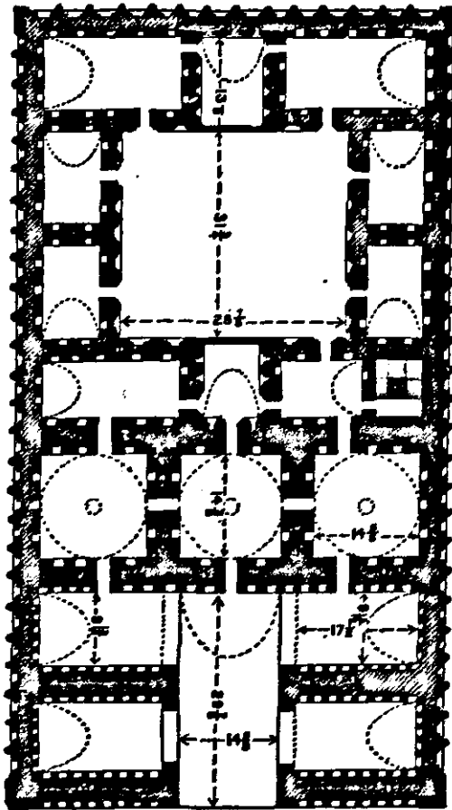
GROUND PLAN OF THE PALACE AT FIRUZABAD (after Perrot). N.B.—The dimensions are in English yards.
