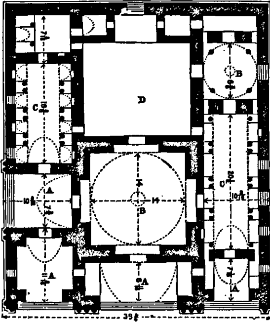
GROUND PLAN OF THE SERISTAN PALACE (after Flindin).
