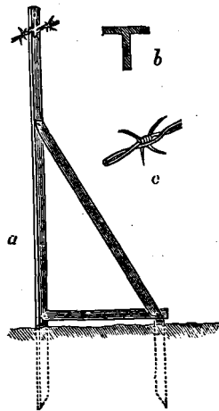
a. Standard in position in the fence. b. Cross section of the steel bar forming the upright. c. Section of the twisted steel wire, showing barb fastenings.
