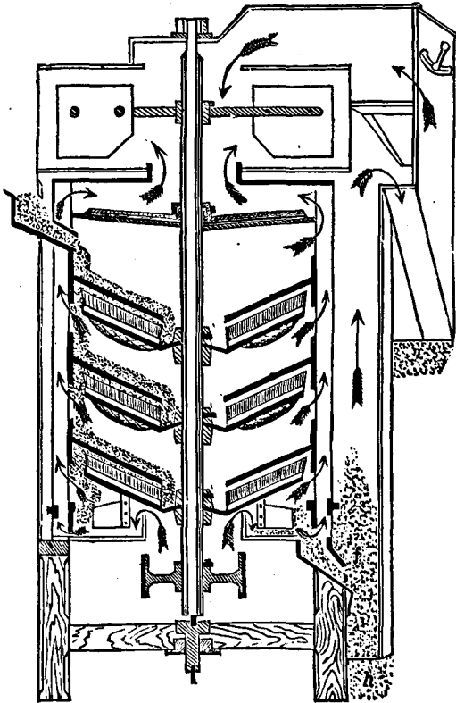
FIG. III.— Double Brush Scourer and Polisher.
