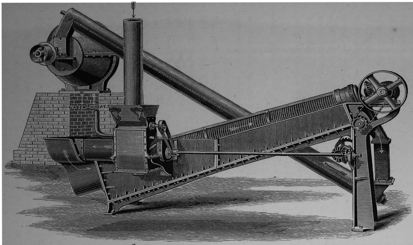
FIG. I.— Wheat Washing and “Whizzing” Machine.
