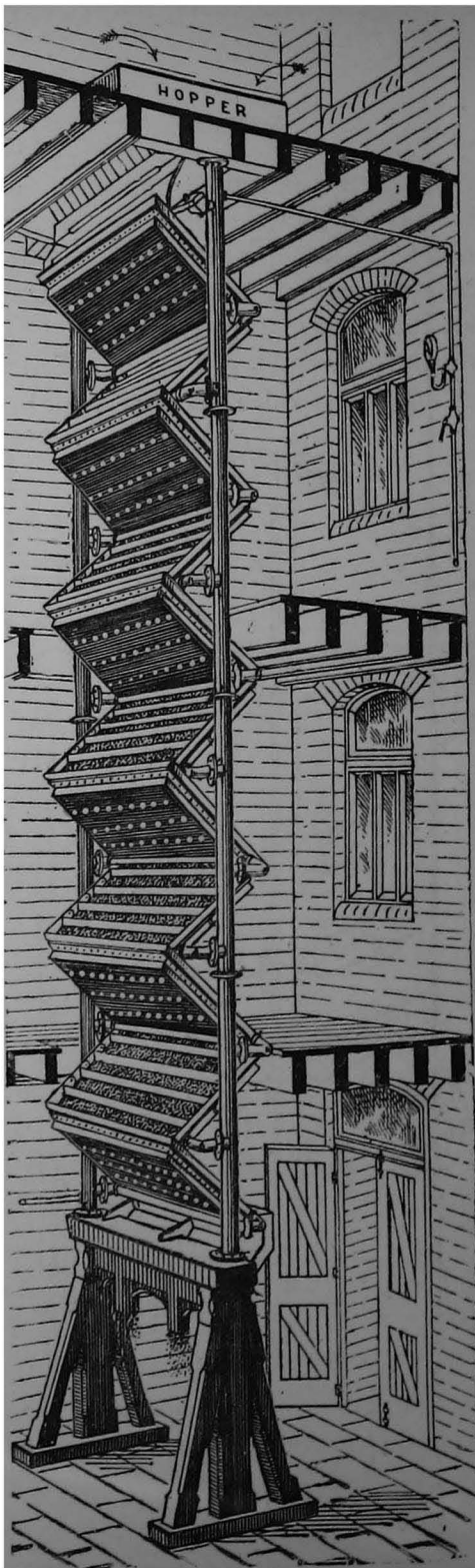
FIG. II.—Automatic Grain Drier and Conditioner.
