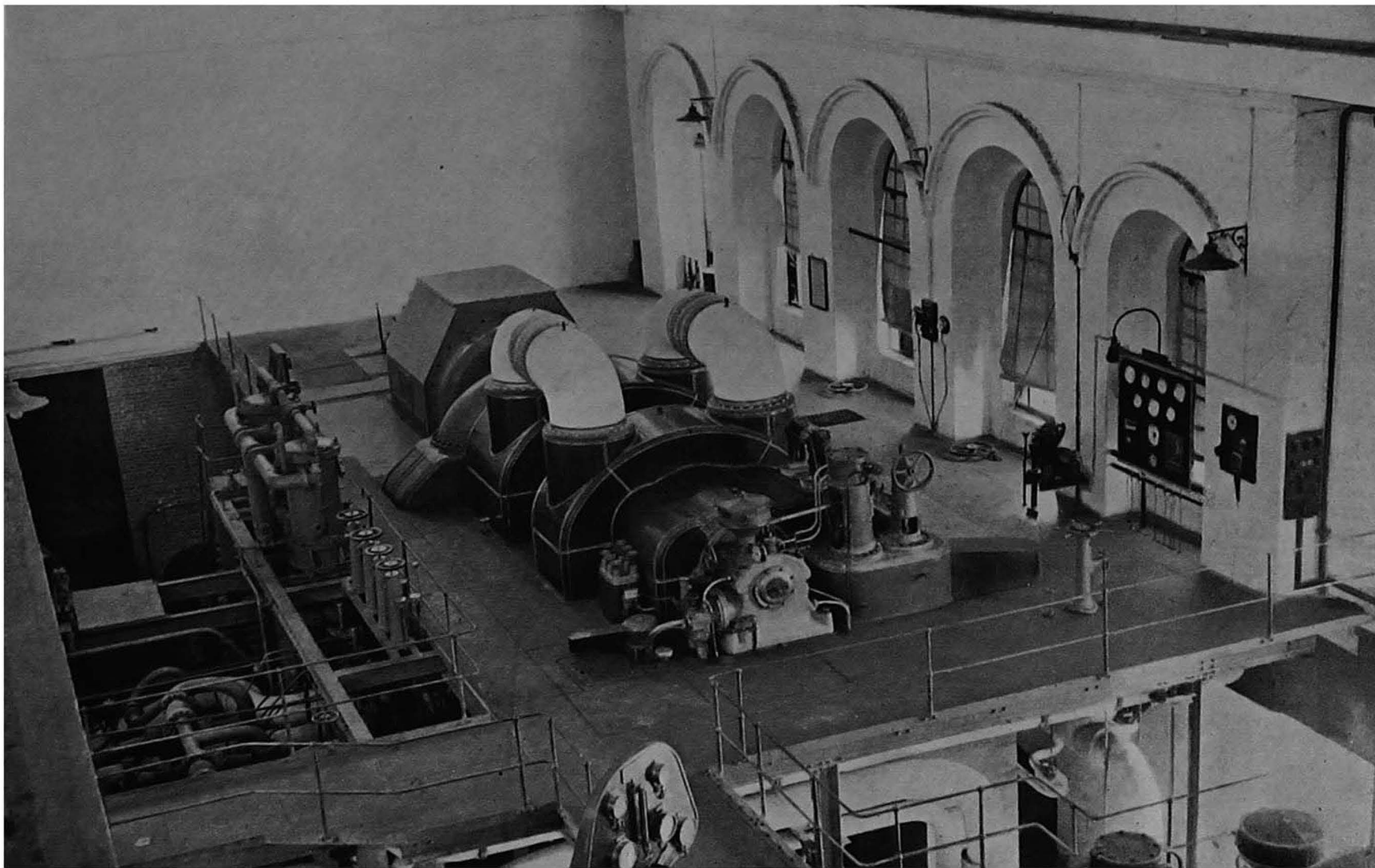
15,000 K. W. set, 400 lbs. sq. inch steam pressure brought into commission in 1937. Cawnpore Electric Supply Corporation, Ltd. (Riverside Power House.)
