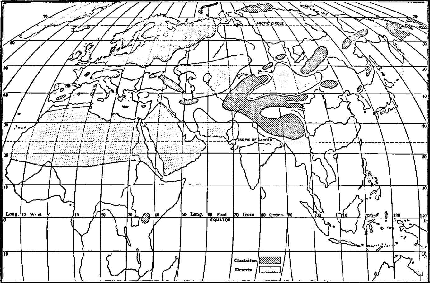
FIG. 1. THE PRESSURE ZONE BETWEEN GLACIATION AND DESERTS.
