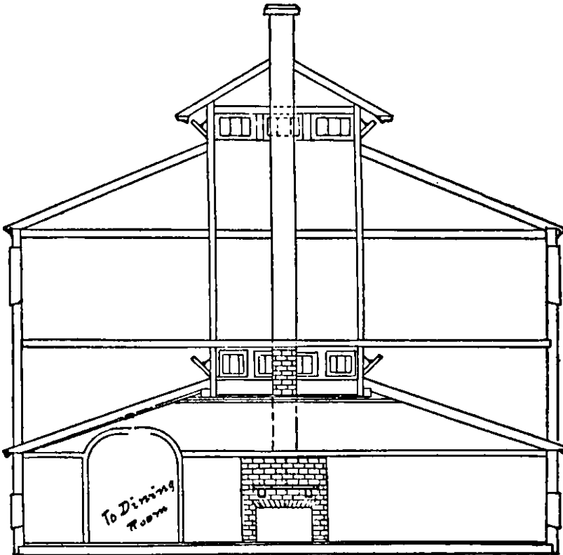
Cross section through living room
