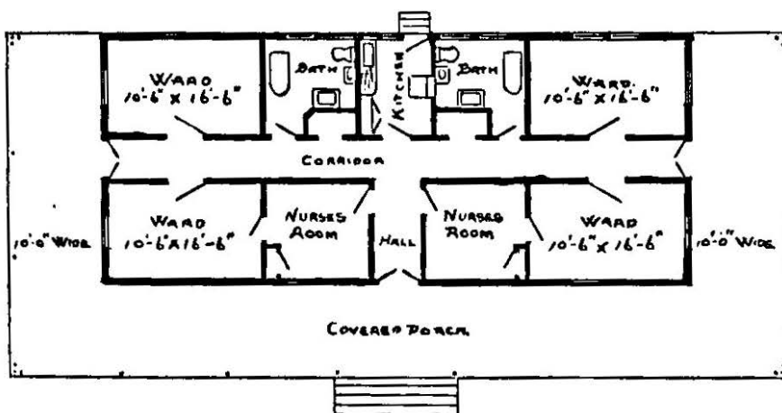
Floor Plan, Surgical Building INDUSTRIAL HOME FOR CRIPPLED CHILDREN, Pittsburgh, Pa. (See page 184)
