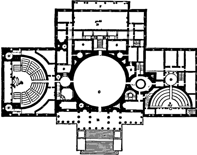
GROUND PLAN OF THE CAPITOL, 1825
