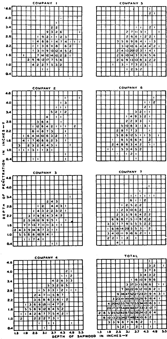
FIG. 21.—QUALITY OF TREATING PROCESS FOR SEVEN PLANTS.
