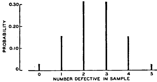
FIG. 121.—CONSUMER'S RISK.
