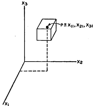
FIG. 16.—QUALITY CONFORMS IF WITHIN VOLUME.
