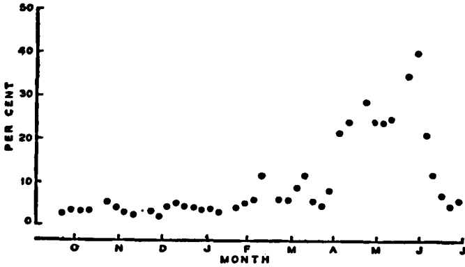
FIG. 145-a.—WHEN DID TROUBLE ENTER?
