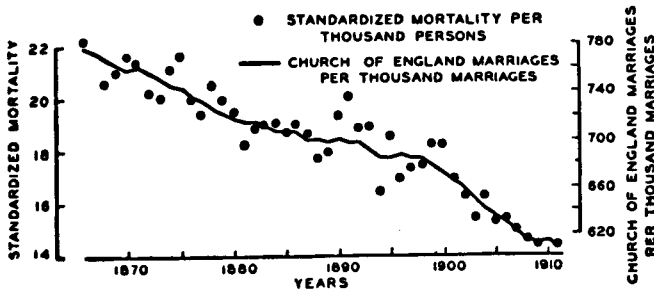
FIG. 82.—EXAMPLE OF A NONSENSE CORRELATION.
