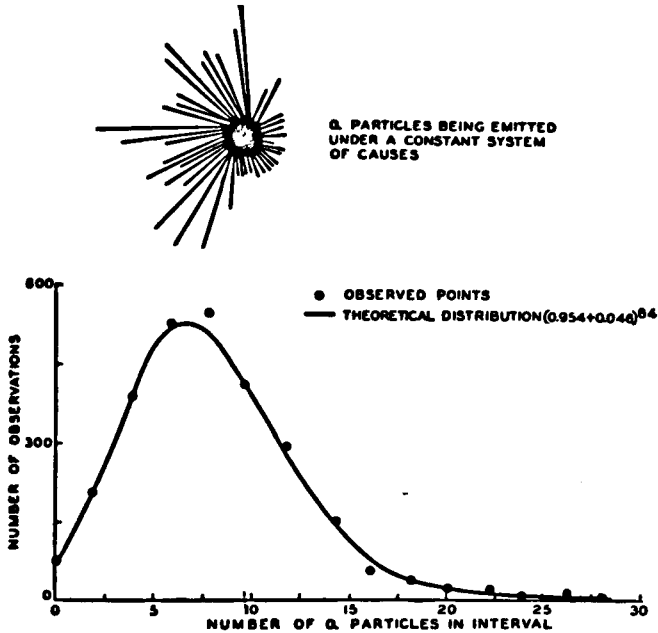
FIG. 43.—FREQUENCY DISTRIBUTION OF ALPHA PARTICLES.
