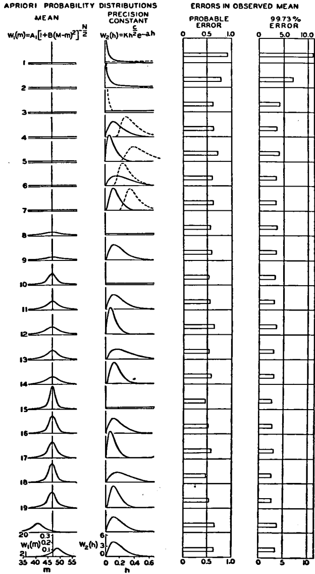
FIG. 130.—SIGNIFICANCE OF a priori EXISTENCE PROBABILITY FUNCTIONS.
