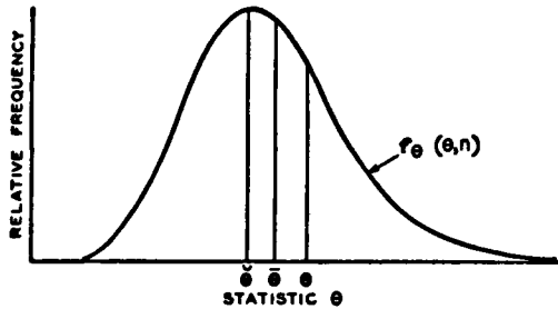
FIG. 97.—SCHEMATIC ASYMMETRICAL DISTRIBUTION OF A STATISTIC.
