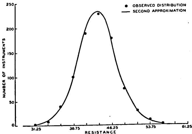
FIG. 118.—TROUBLE REMOVED—CRITERION V GIVES NEGATIVE TEST.
