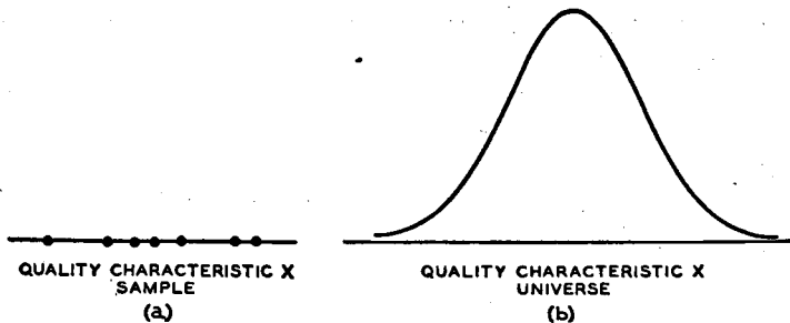
FIG. 23.—SCHEMATIC RELATION BETWEEN SAMPLE AND UNIVERSE.
