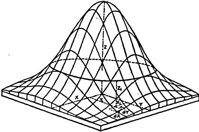
FIG. 35.—THE NORMAL SURFACE.
