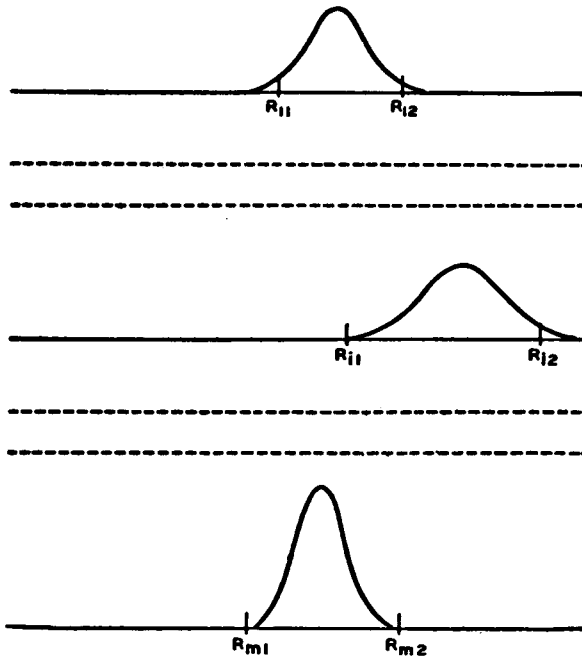
FIG. 86.—TOLERANCE RANGES ON OBSERVED DISTRIBUTIONS.
