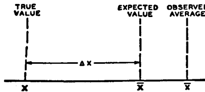
FIG. 132.—PROBLEM OF ELIMINATING ERRORS OF MEASUREMENT.
