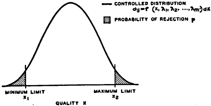
FIG. 85.—TOLERANCE ON FRACTION DEFECTIVE FOR CONTROLLED QUALITY.
