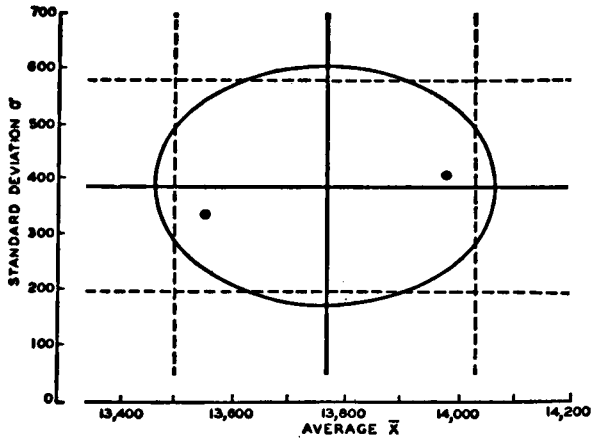
FIG. 106.—TESTS FOR CONTROL.
