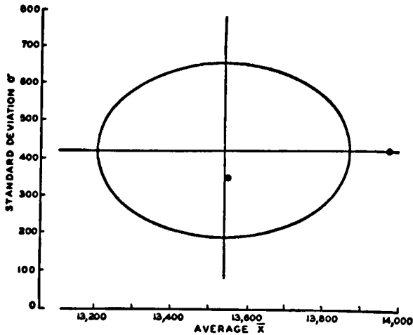
FIG. 104.—ANOTHER CONTROL CHART TEST.
