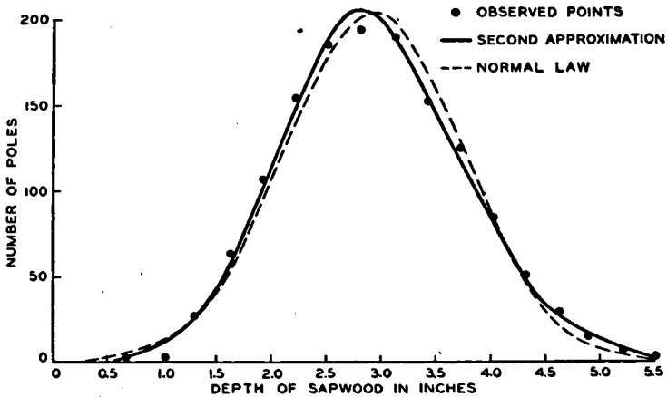
FIG. 32.—SIGNIFICANCE OF AVERAGE, STANDARD DEVIATION, AND SKEWNESS.
