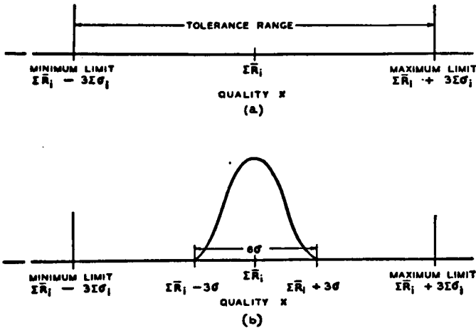
FIG. 87.—ILLUSTRATING PROPER WAY TO SET LIMITS.
