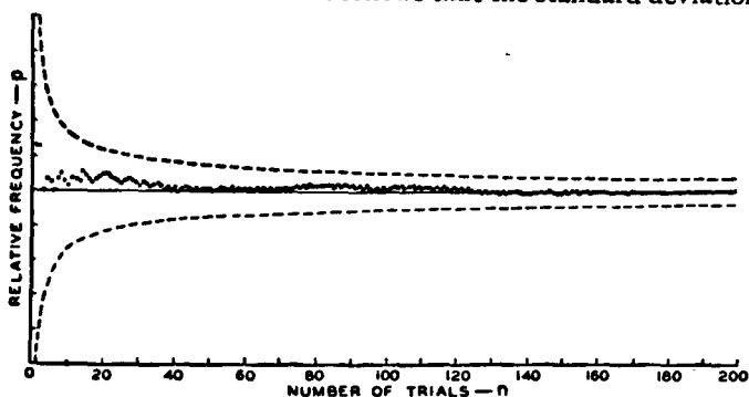
FIG. 127- b .—BASIC INFORMATION FOR STATISTICAL PREDICTION.
