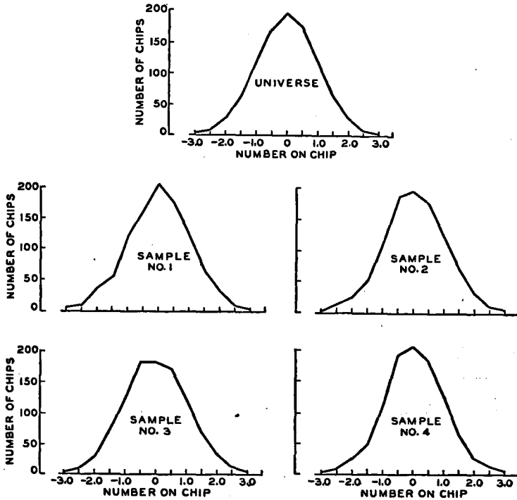
FIG. 56.—SAMPLING FLUCTUATIONS UNDER CONTROLLED CONDITIONS.
