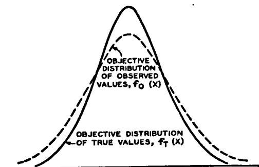
FIG. 134.—EFFECT OF ERROR OF MEASUREMENT.
