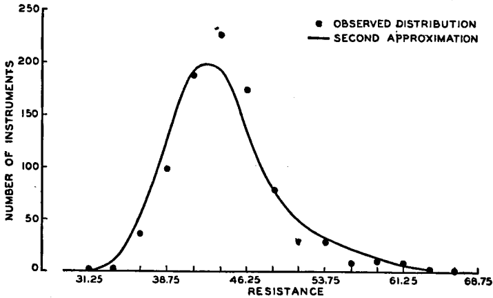
FIG. 117.—CRITERION V GIVES POSITIVE TEST, INDICATING TROUBLE.
