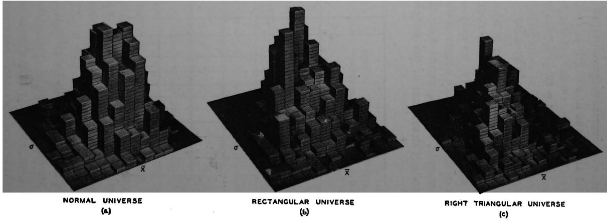
FIG. 64.—OBSERVED FREQUENCY SURFACE HISTOGRAMS SHOWING CORRELATION BETWEEN THE AVERAGE AND STANDARD DEVIATION IN SAMPLES OF SIZE n = 4 .
