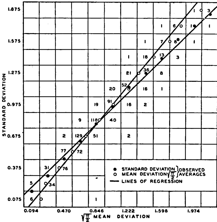
FIG. 99.—CORRELATION BETWEEN STANDARD DEVIATION AND \sqrt{\frac{\pi}{2}} TIMES MEAN DEVIATION FOR SAMPLES OF FOUR FROM A NORMAL UNIVERSE.
