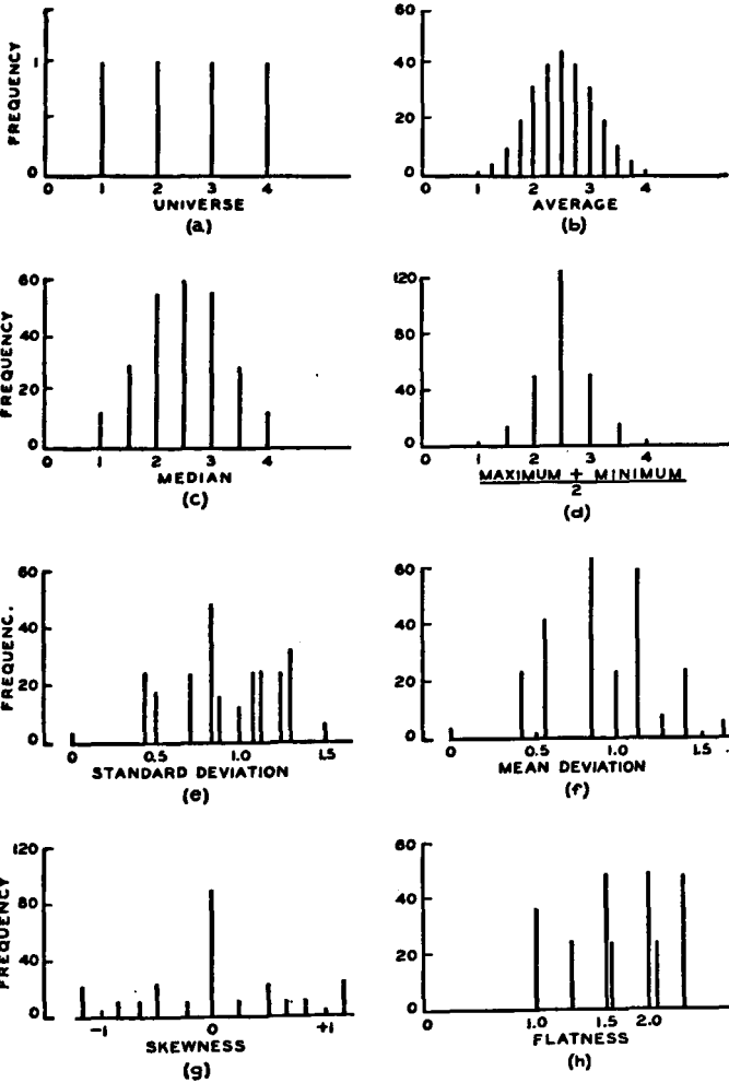
FIG. 57.—DISTRIBUTION OF STATISTICS FOR SAMPLES SHOWN IN TABLE 25.
