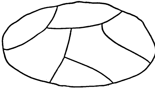
FIG. 144.—SCHEMATIC OF DIVISION INTO RATIONAL SUBGROUPS.
