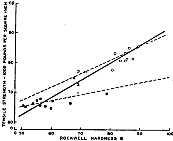
FIG. 79.—EFFECT OF SPURIOUS CORRELATION.
