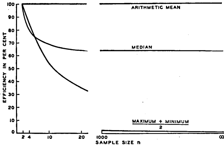
FIG. 96.—EFFICIENCY OF THE MEDIAN AND \frac{\text{MAX.} + \text{MIN.}}{2} AS A FUNCTION OF SAMPLE SIZE n .
