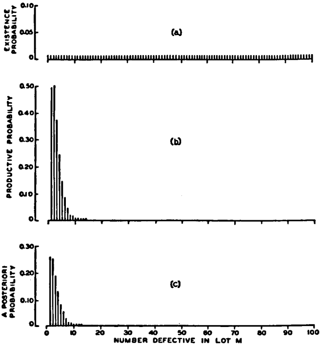
FIG. 122.—RELATION BETWEEN PROBABILITIES.
