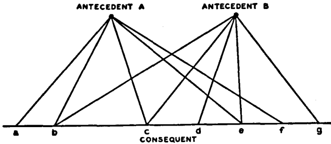
FIG. 129.—SCHEMATIC OF CAUSAL RELATIONSHIP.
