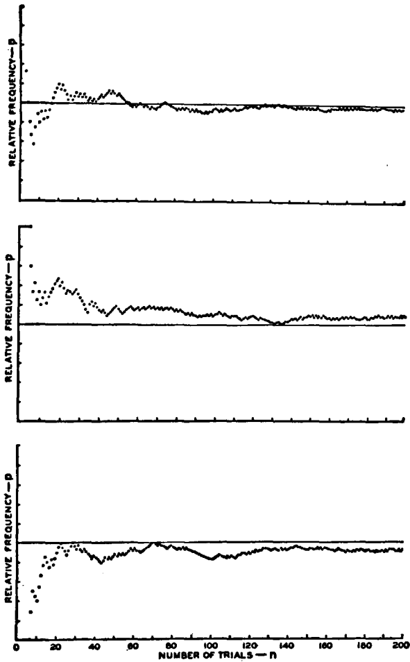
FIG. 128.—BASIC INFORMATION FOR STATISTICAL PREDICTION.
