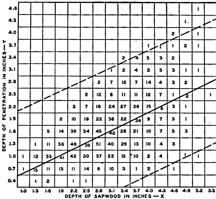
FIG. 38.—LINE OF REGRESSION AND 99.7 PER CENT LIMITS.
