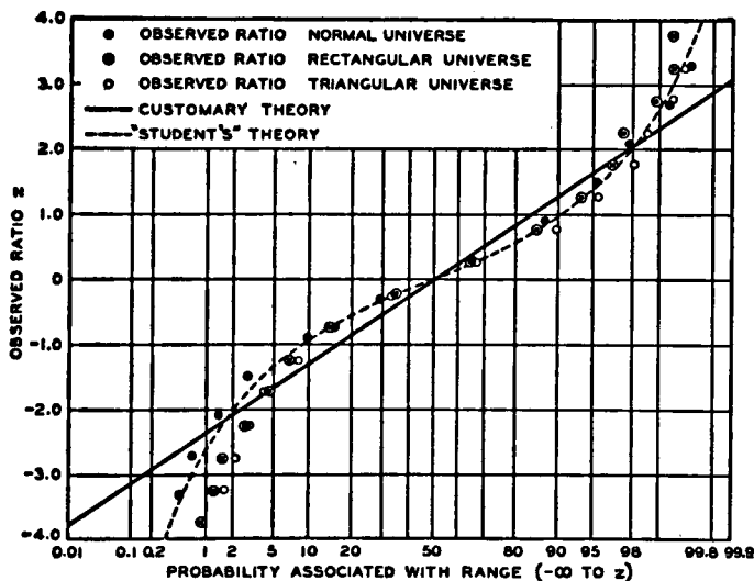
FIG. 63.—PROBABILITY ASSOCIATED WITH RANGE ( -\infty TO z ).
