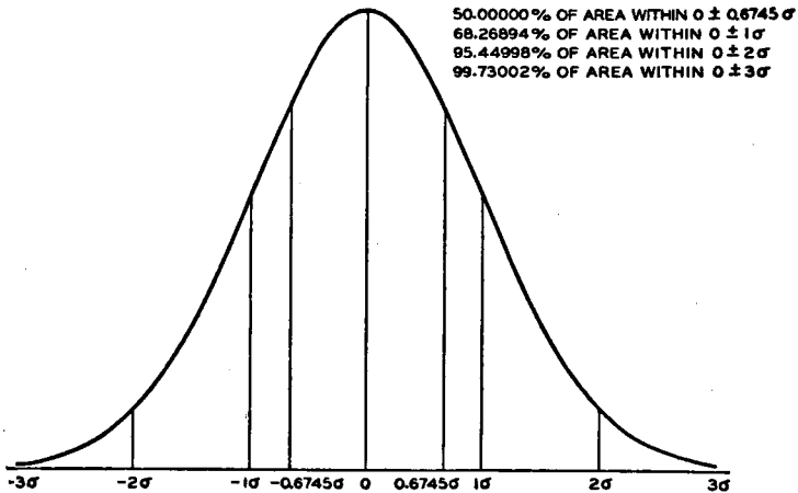
FIG. 33.—NORMAL LAW CURVE.
