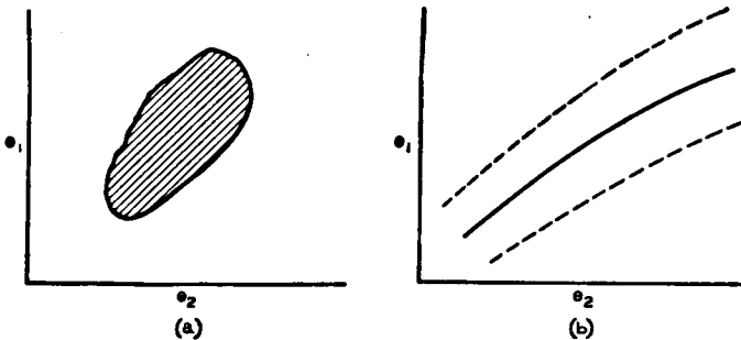
FIG. 101.—TWO TYPICAL FORMS OF CONTROL CHART.
