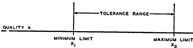
FIG. 83.—RELATIONSHIP BETWEEN TOLERANCE RANGE AND TOLERANCE LIMITS.
