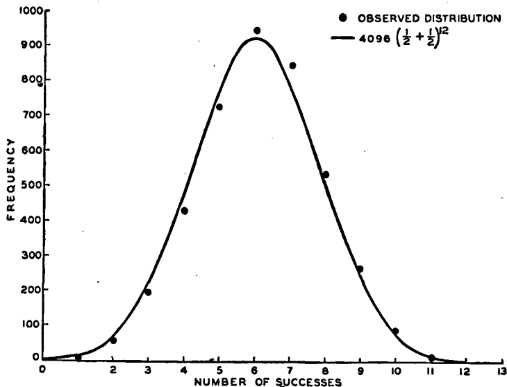
FIG. 120.—THE FACT THAT THE SMOOTH THEORETICAL CURVE APPEARS TO BE SHIFTED TO THE LEFT SUGGESTS LACK OF CONTROL EVEN THOUGH CRITERION V GIVES NEGATIVE TEST.
