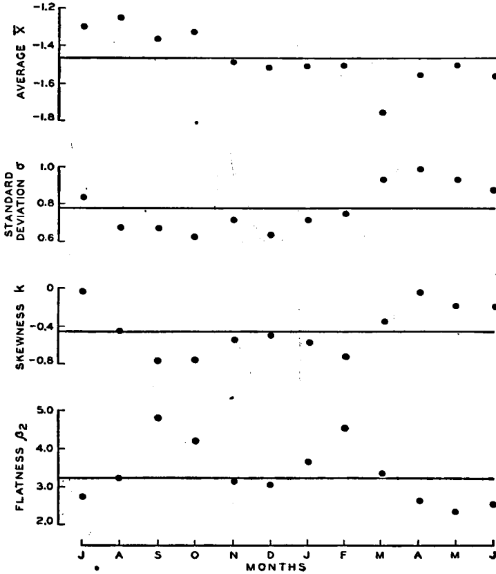
FIG. 20.—QUALITY RECORD IN TERMS OF STATISTICS.
