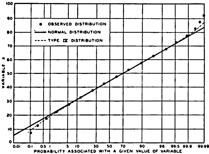
FIG. 93.—GRAPHICAL PRESENTATION OF DATA IN TABLE 40.
