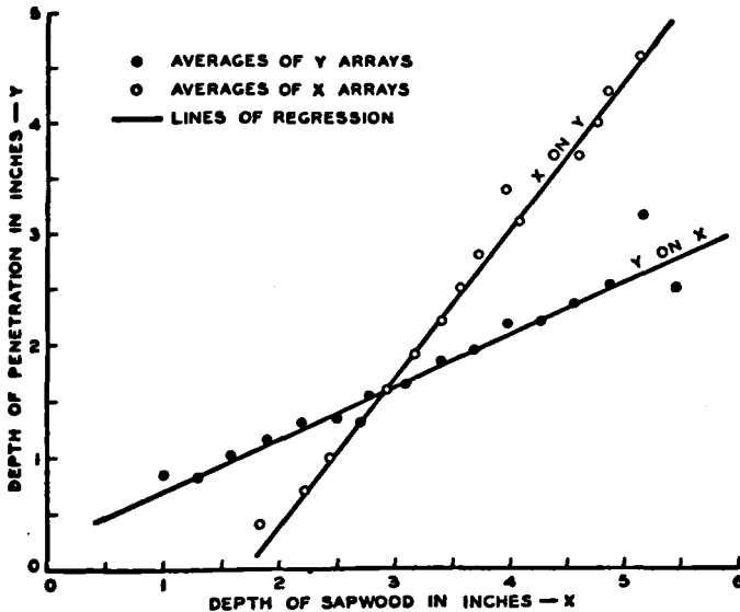
FIG. 37.—LINES OF REGRESSION.
