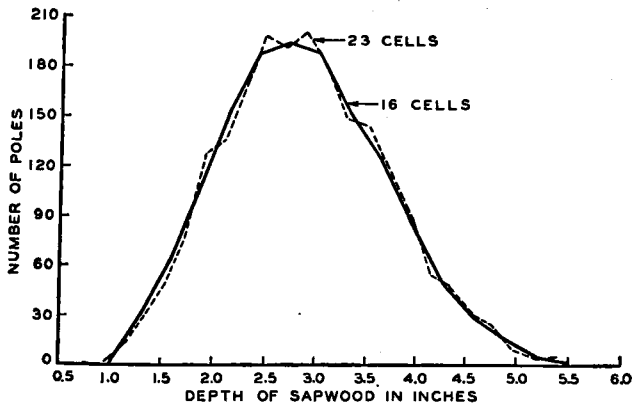
FIG. 28.—EFFECT OF CLASSIFICATION ON GRAPHICAL REPRESENTATION.
