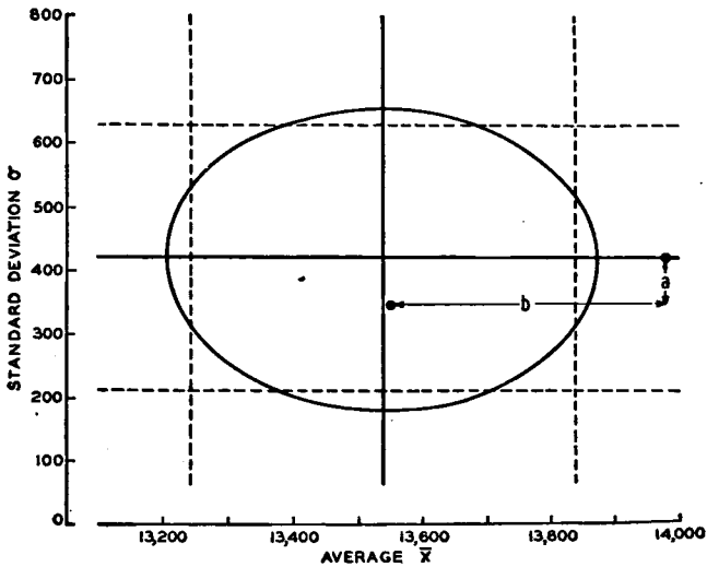
FIG. 105.—COMPARISON OF THREE TESTS.
