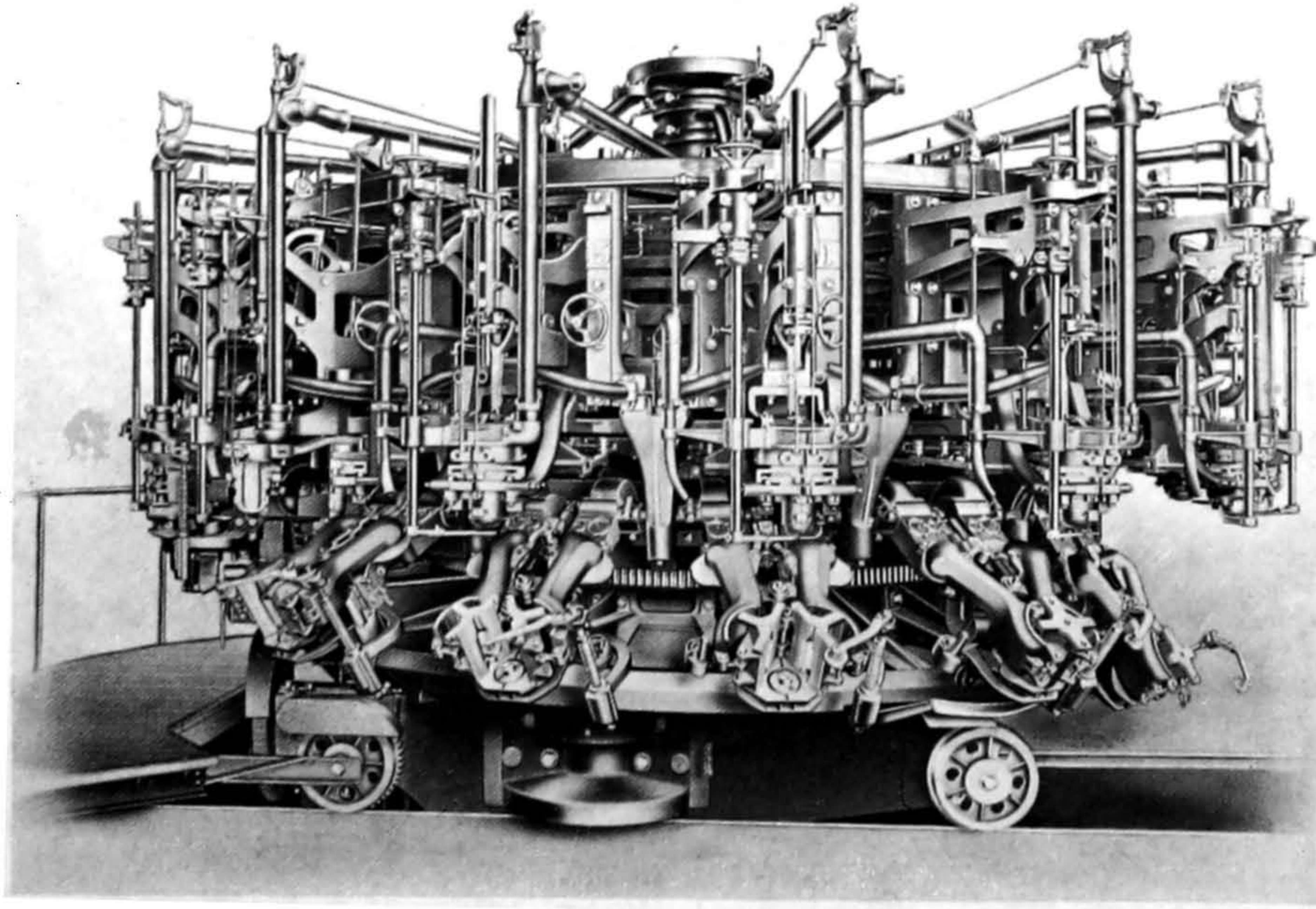
AN AUTOMATIC BOTTLE-MAKING MACHINE, MADE UNDER PATENTS ISSUED 1904-16
