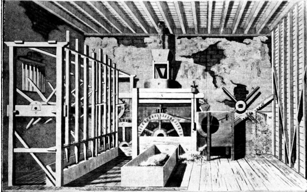
A RICE MILL IN SOUTH CAROLINA, EARLY NINETEENTH CENTURY
