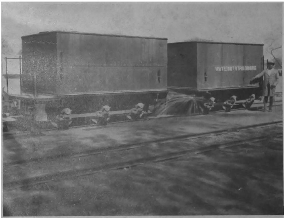
Water Trucks (used for watering the unballasted track between Muttra Cantonment and Brindavan—a distance of 6 miles—to eliminate the dust nuisance).
